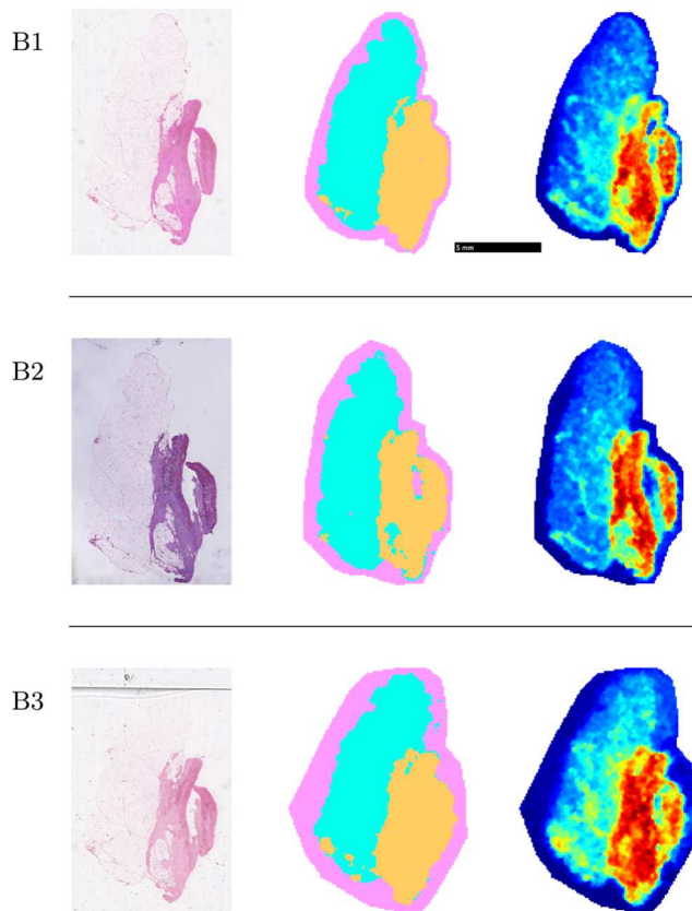
FIG. 5. H&E stains (left column), cluster maps (center column), and DIPPS maps for the cancer cluster (right column) for the three datasets B1, B2, and B3 (each represented in a row). Note that n_{a^*} = 173,117,111 m/z bins are visualized in the DIPPS maps for the datasets B1, B2, and B3, respectively.
