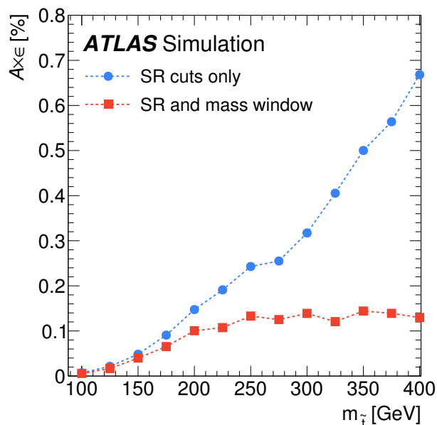
Figure 5. Total acceptance times efficiency ( A \times \epsilon ) of the SR cuts of eq. (5.3), and SR cuts combined with the mass window selection in table 1, as a function of m_{\tilde{t}} . The denominator of the efficiency (in %) is the total number of events, i.e. the top row in table 3.
