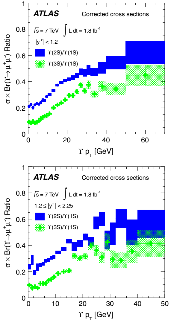
FIG. 19 (color online). Ratios of differential Y(2S)/Y(1S) and Y(3S)/Y(1S) cross sections multiplied by the dimuon branching fractions versus Y p_T in the (top) central and (bottom) forward rapidity regions. Points with error bars indicate results of the measurements with statistical uncertainties while shaded areas correspond to total uncertainties on each point, including systematic effects, but excluding spin-alignment effects.
