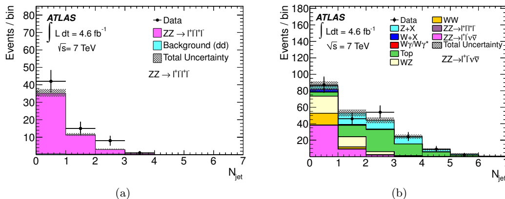
Figure 4. (a) Jet multiplicity for the ZZ \rightarrow \ell^+\ell^-\ell'^+\ell'^- selection and (b) jet multiplicity for the ZZ \rightarrow \ell^+\ell^-\nu\bar{\nu} selection (with all selections applied but the jet veto). The points represent the observed data. In (a) the ZZ \rightarrow \ell^+\ell^-\ell'^+\ell'^- background is normalized to the data-driven (dd) estimate, while in (b) the histograms show the prediction from simulation. The shaded band shows the combined statistical and systematic uncertainty on the prediction.
