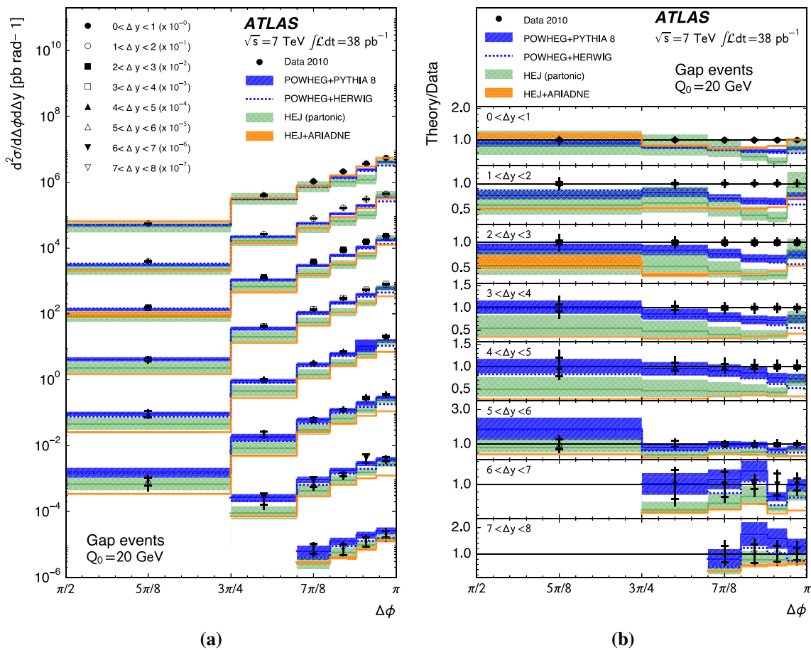
Fig. 8 The measured double-differential cross sections as a function of \Delta\phi for eight slices in \Delta y , for gap events. The veto scale is Q_0 = 20 \text{ GeV} . For comparison, the HEJ, HEJ+ARIADNE,
