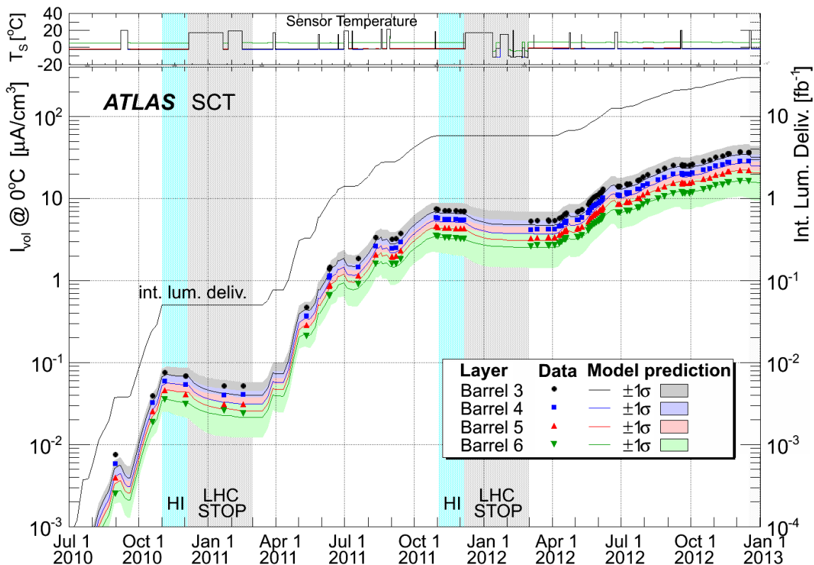
Figure 30. Comparison between data (points) and Hamburg/Dortmund model predictions (lines with uncertainties shown by the coloured bands) of the leakage current per unit volume at 0°C ( I_{vol} ) of the four barrel layers. The integrated luminosity and the average sensor temperatures are also shown. The blue shading and label ‘HI’ indicate periods of heavy-ion running, while extended periods with no beam in the LHC during which the SCT was off are shaded grey.
