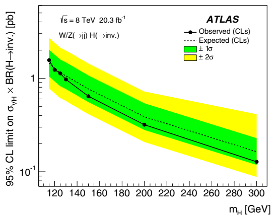
Fig. 6 Upper limits on \sigma_{VH} \times BR(H \rightarrow \text{inv.}) at 95 % CL for a Higgs boson with 115 < m_H < 300 GeV. The full and dashed lines show the observed and expected limits, respectively
