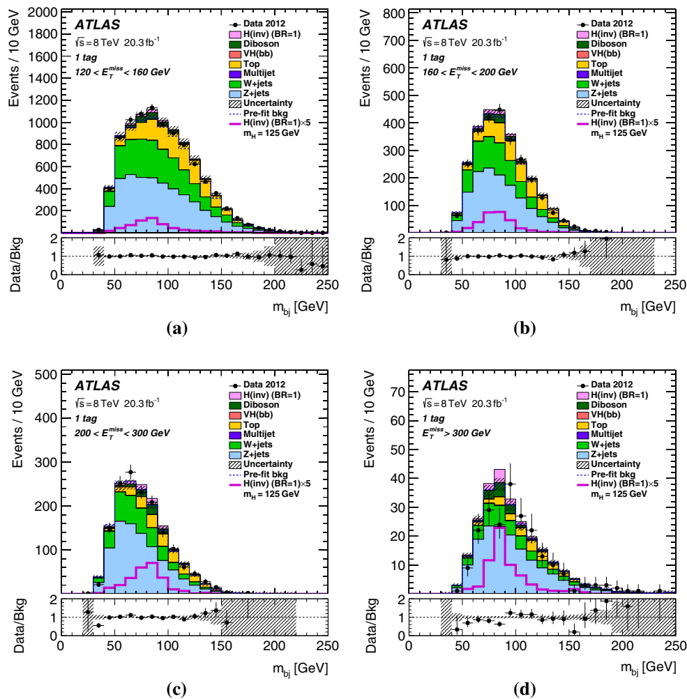
Fig. 4 The dijet invariant mass ( m_{bj} ) distributions in the signal region for the 1- b -tag category, for events with E_T^{miss} in the range a (120–160 GeV), b (160–200 GeV), c (200–300 GeV) and d (>300 GeV). The data are compared with the background model after the likelihood fit. The bottom plots show the ratio of the data to the total background.
