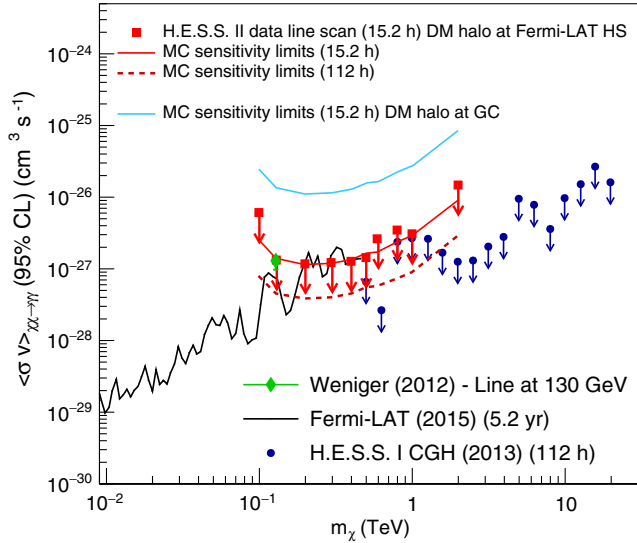
FIG. 3. \langle\sigma v\rangle limits at 95% C.L. (red points) for the line scan between 100 GeV and 2 TeV, derived from 15.2 h of data and using an Einasto DM profile with a \Phi value calculated with the CLUMPY package [25] ( \rho_s = 20 kpc, r_s = 0.17 ). The MC estimations are presented with the same conventions as in Fig. 2. The former limits from H.E.S.S. I [3] obtained in the CGH region and the Fermi LAT [10] are represented by blue and black data points, respectively. The \langle\sigma v\rangle value corresponding to the 130 GeV line feature reported as R16 in Ref. [7] is shown in green. The limits extracted with the assumption of the DM halo position at the GC are shown with a continuous blue line (see the text). It should be noted that the comparison of the limits on the hot spot obtained in this work cannot be directly done with the H.E.S.S. I results as the DM halo was centered on the Galactic Center position in the sky. In case of the Fermi LAT, the red curve can still be compared to the Fermi LAT limits as the latter would only be marginally modified (at the level of 1%) by the displacement of the DM halo, given the very large size of the ROI ( 16^\circ of radius) in use.
