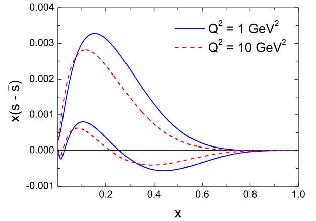
Fig. 4. Strange quark asymmetry x(s - \bar{s}) at Q^2 = 1 GeV 2 (solid blue curves) and evolved to Q^2 = 10 GeV 2 (dashed red curves). The upper (lower) curves correspond to the maximum (minimum) value for S^- = 1.12 \times 10^{-3} ( -0.07 \times 10^{-3} ), for cutoff parameters \mu_1 = 526 MeV, \mu_2 = 894 MeV ( \mu_1 = 545 MeV, \mu_2 = m_K ).
