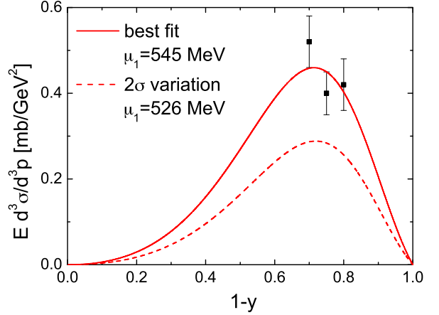
Fig. 2. Differential cross section for the best fit to the pp \rightarrow \Lambda X data [49] in the region y < 0.35 (solid curve, \mu_1 = 545 MeV), as a function of 1 - y for k_{\perp} = 75 MeV, and for a fit 2\sigma below the central values (dashed curve, \mu_1 = 526 MeV).
