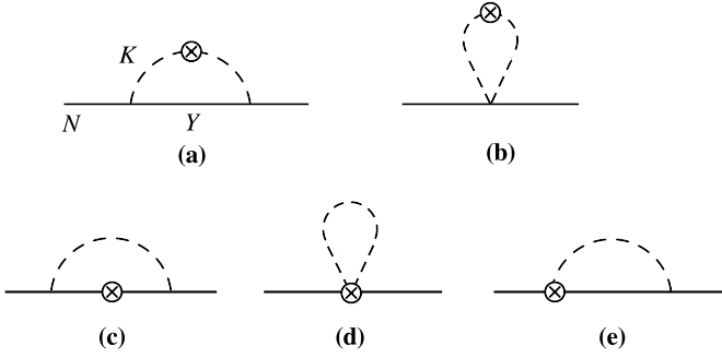
Fig. 1. Loop contributions to the \bar{s} PDF from (a) kaon rainbow and (b) kaon bubble diagrams, and to the s -quark PDF from (c) hyperon rainbow, (d) tadpole, and (e) Kroll–Ruderman diagrams. Nucleons N and hyperons Y = \Lambda, \Sigma are denoted by external and internal solid lines, respectively, and kaons K by dashed lines, with crosses \otimes representing insertions of the vector current. The Kroll–Ruderman diagram with a current insertion on the right-hand vertex is not shown.
