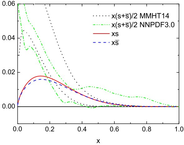
Fig. 3. Comparison between the strange x_s (solid red curve) and antistrange x_{\bar{s}} (dashed blue curve) PDFs from kaon loops, for the cutoff parameters ( \mu_1 = 545 MeV and \mu_2 = 600 MeV) that give the maximum total s + \bar{s} , with the upper and lower limits of the error bands for x(s + \bar{s})/2 at Q^2 = 1 GeV 2 from the MMHT14 [51] (black dotted) and NNPDF3.0 [52] (green dot-dashed) global fits.
