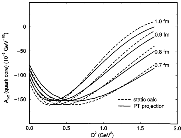
FIG. 3. The effect of the center of mass correction on the helicity amplitude A_{3/2} for the bare bag. The number on each curve indicates the bag radius in fm for the calculation.
