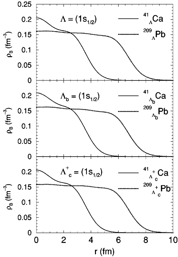
FIG. 1. Total baryon density distributions in {}^{41}_j\text{Ca} and {}^{209}_j\text{Pb} ( j = \Lambda, \Lambda_c^+, \Lambda_b ), for the 1s_{1/2} configuration for the \Lambda , \Lambda_c^+ , and \Lambda_b .
