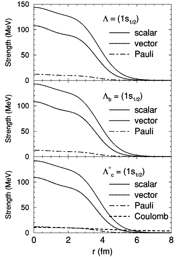
FIG. 2. Potential strengths for the 1s_{1/2} state felt by the \Lambda , \Lambda_c^+ , and \Lambda_b in {}^{41}_j\text{Ca} ( j = \Lambda, \Lambda_c^+, \Lambda_b ). “Pauli” stands for the effective, repulsive, potential representing the Pauli blocking at the quark level plus the \Sigma_{c,b}N-\Lambda_{c,b}N channel coupling, introduced at the baryon level phenomenologically [10].
