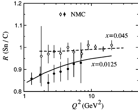
FIG. 1. Q^2 variation of the Sn/C structure function ratio in the model of Ref. [14] for x=0.0125 (solid) and x=0.045 (dashed). The data are from NMC [11], with statistical and systematic errors added in quadrature.
