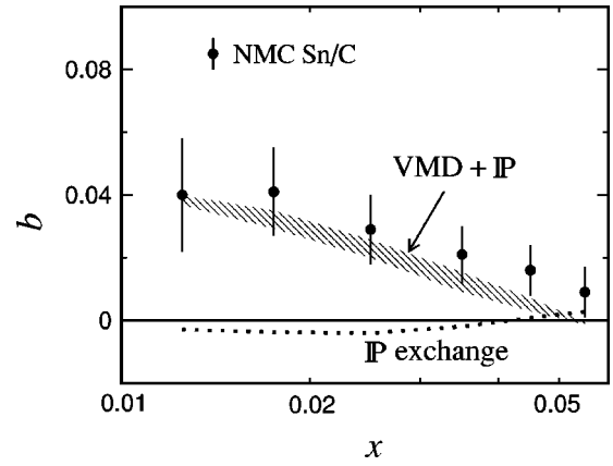
FIG. 2. Logarithmic slope b in Q^2 of the NMC Sn/C ratio as a function of x [11], compared with the nuclear shadowing model of Ref. [14]. The statistical and systematic errors are added in quadrature.
