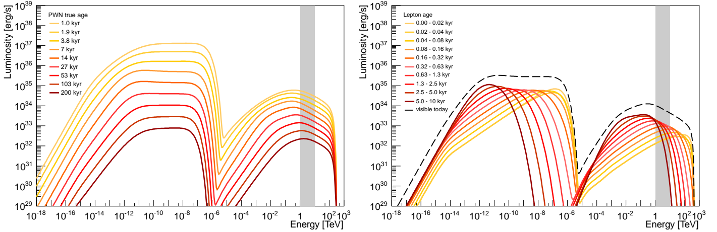
Fig. A.1. Modelled spectral energy distribution (SED) of a generic PWN with parameters according to baseline model given in Table A.1. See Appendix A.7 for caveats of the SEDs. Left : time evolution of the SED, ranging from 1 kyr to 200 kyr. Right : decomposition of the SED of a middle-aged PWN (10 kyr; black dashed curve) into contributions by leptons from various injection epochs (coloured lines). The grey-shaded bands indicate the energy range of 1–10 TeV explored in this paper.
