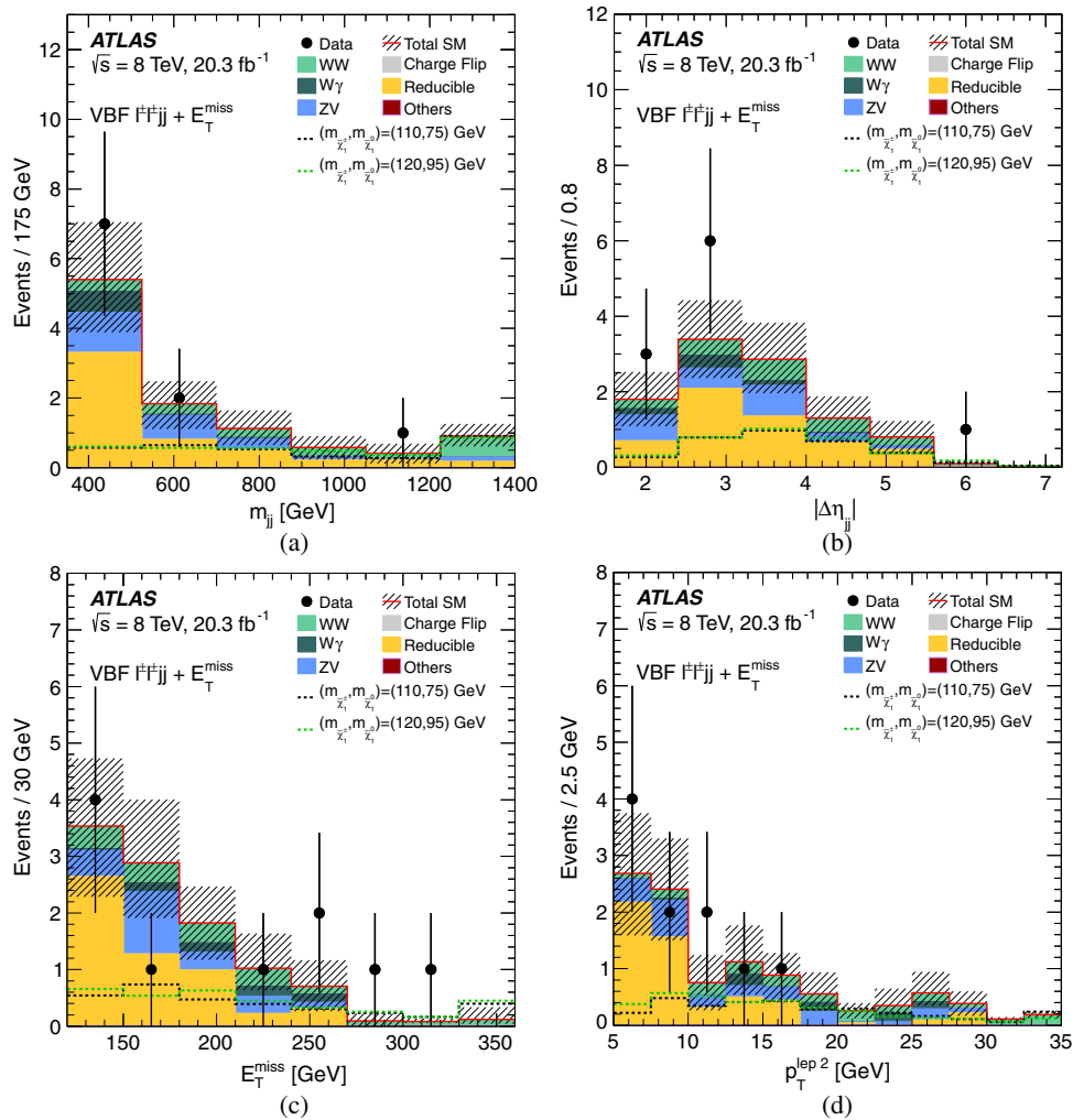
FIG. 11. For events in the same-sign VBF signal region, the (a) m_{jj} , (b) separation in \eta between the two leading jets |\Delta\eta_{jj}| , (c) E_T^{\text{miss}} , and (d) p_T^{\text{lep } 2} in SR2 \ell -2. The “Others” background category includes t\bar{t}V + tZ , VVV , and SM Higgs boson production. The uncertainty band includes both the statistical and systematic uncertainties on the SM prediction. The last bin in each distribution includes the overflow.
