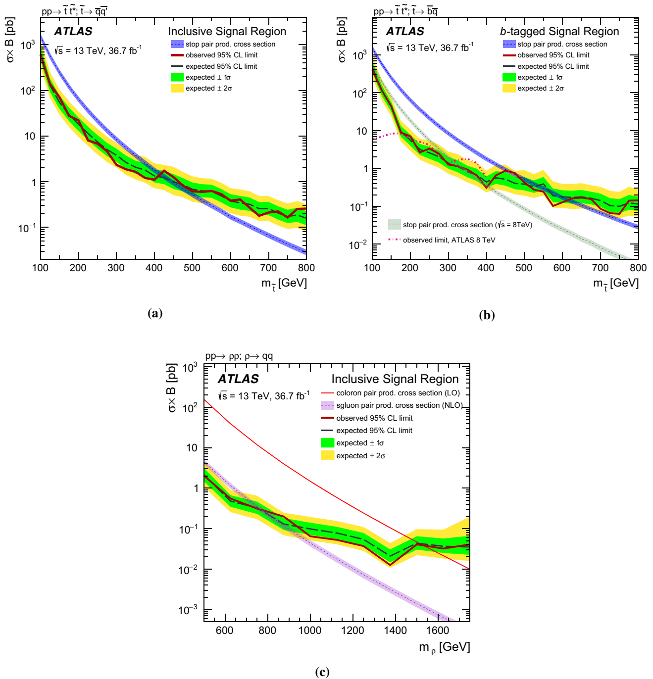
Fig. 9 The 95% CL upper limit on the \sigma \times B value compared to the theoretical cross-section for the direct pair-production of top squarks with decays into a \bar{q} \bar{q}' or b \bar{b} \bar{s} and c high-mass colorons decaying into qq and sgluons decaying into gg . The dashed black and solid red lines show the 95% CL expected and observed limits respectively, including all uncertainties except the theoretical signal cross-section uncertainty.
