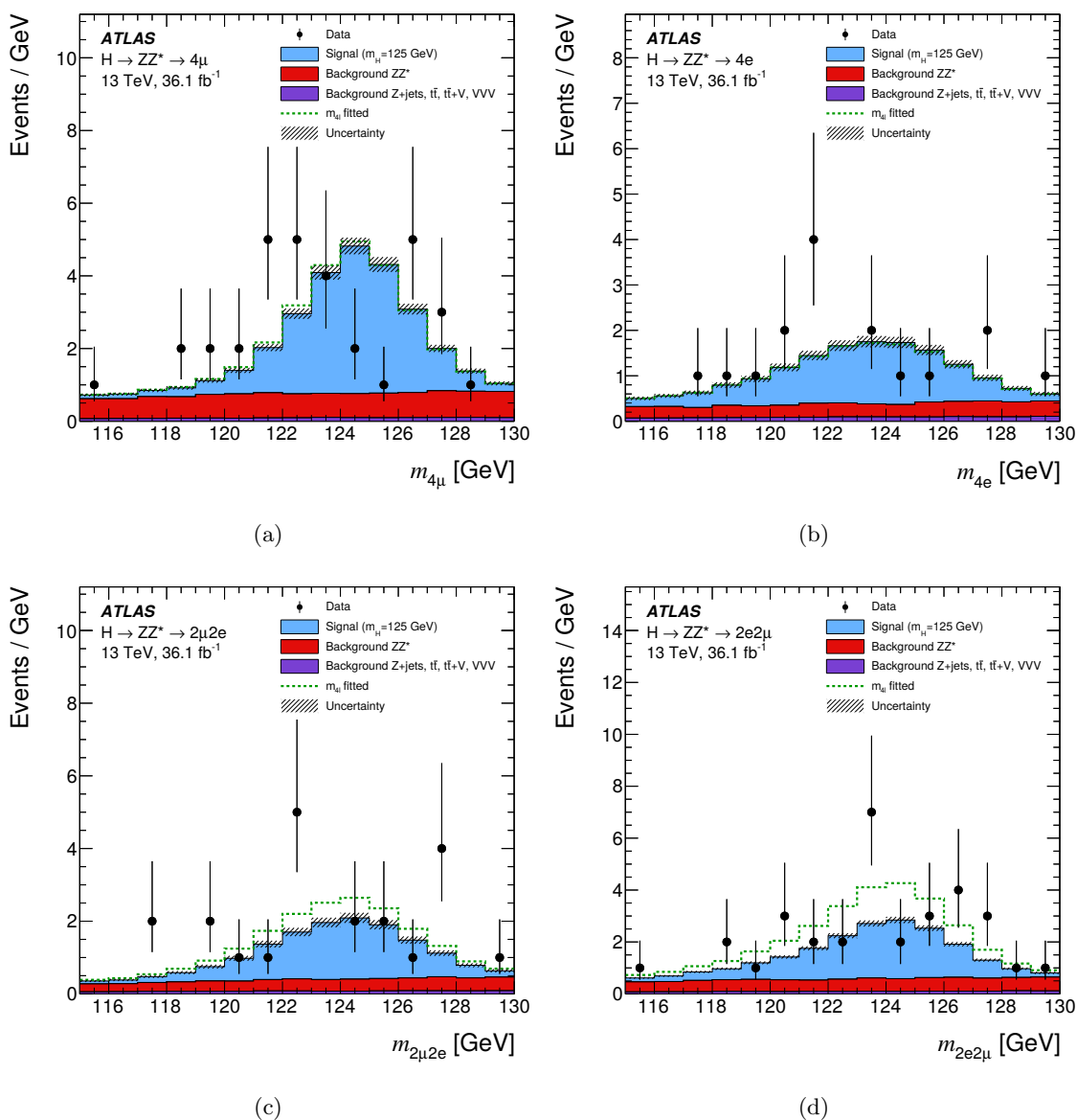
Figure 4. Template fit of SM Higgs boson signal and background to the data for the inclusive distributions for the different decay channels (a) 4\mu , (b) 4e , (c) 2\mu 2e , (d) 2e2\mu . The error bars on the data points indicate the statistical uncertainty. The SM Higgs boson predictions are normalized to the cross sections discussed in section 3, while the backgrounds are normalized to the estimates described in section 6. The uncertainty in the prediction is shown by the dashed band. The dotted green line illustrates the best fit.
