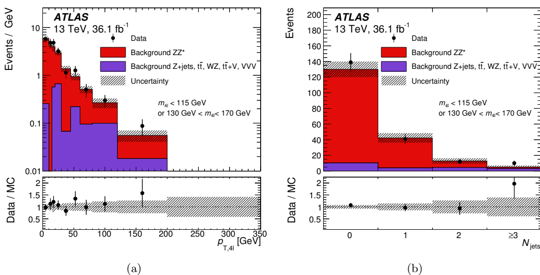
Figure 2. Reconstructed event yields in bins of (a) the transverse momentum of the four leptons p_{T,4\ell} and (b) the number of jets N_{jets} , in a non-resonant ZZ^* -enriched control region, obtained by applying the full event selection except for the m_{4\ell} window, i.e. m_{4\ell} < 115 \text{ GeV} or 130 \text{ GeV} < m_{4\ell} < 170 \text{ GeV} . The error bars on the data points indicate the statistical uncertainty. The uncertainty in the prediction is shown by the dashed band. The bottom part of the figures shows the ratio of data to the MC expectation.
