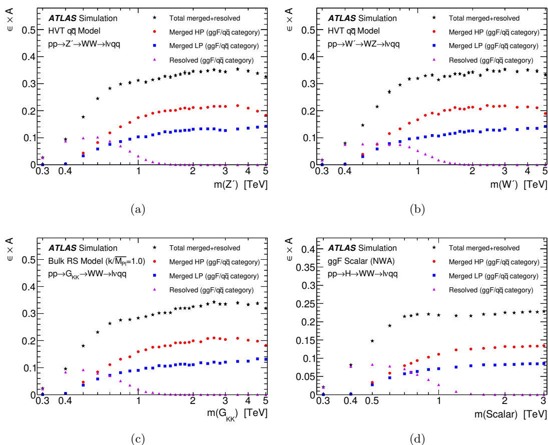
Figure 3. The product of signal efficiency ( \epsilon ) and acceptance ( A ) is presented in the ggF/q \bar{q} category for signals produced via ggF or q \bar{q} fusion. The \epsilon \times A is presented for HVT (a) WW \rightarrow lvqq , (b) HVT WZ \rightarrow lvqq , (c) RS G_{KK} \rightarrow lvqq and (d) neutral scalar signal ( H ) decaying into lvqq in the narrow-width approximation (NWA) in the various analysis categories. It is defined as the ratio of the number of signal events reconstructed in the signal region to the number of generated signal events.
