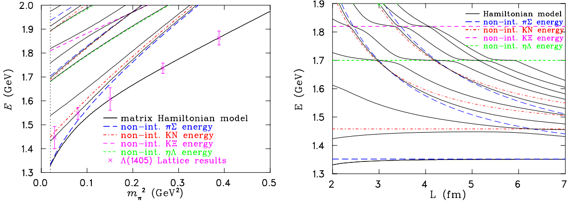
Figure 1: (left) The quark-mass dependence ( m_q \propto m_\pi^2 ) of the lowest-lying \Lambda(1405) states observed in our lattice QCD calculations [1] is illustrated by the discrete points at each of the pion masses available in the PACS-CS ensembles. The low-lying energy spectrum of our Hamiltonian model (solid curves) constrained to the Lattice QCD results (discrete points) is also illustrated. The associated non-interacting meson-baryon basis states are illustrated by the dashed curves. (right) The volume dependence of the spin-1/2 odd-parity \Lambda spectrum obtained from our Hamiltonian effective field theory analysis of our lattice results at m_\pi = 156 MeV. L denotes the length of the L^3 volume.
