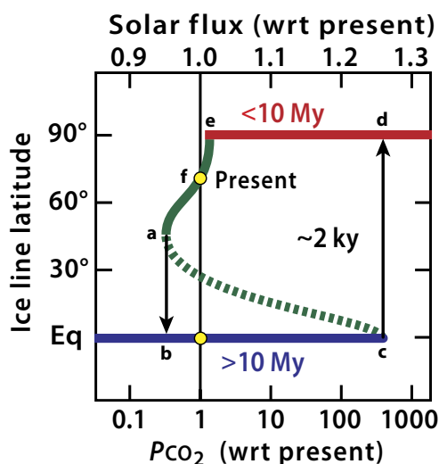
Fig. 1. Generic bifurcation diagram illustrating the Snowball Earth hysteresis.
