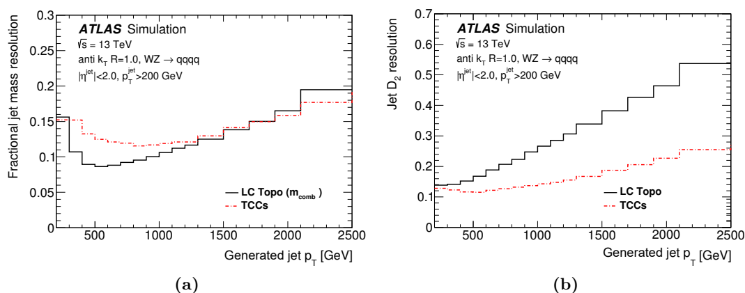
Figure 1. A comparison of (a) the fractional jet mass resolution for jets built from a linear combination of the calorimeter and track-only mass (LC Topo m_{\text{comb}} , solid line), and jets built using combined and neutral Track-CaloClusters objects (dashed lines) as a function of Monte Carlo generator-level jet p_T . The fractional jet resolution of the D_2 variable (b) is compared between Track-CaloClusters and pure calorimeter jets. Only the two jets with the highest p_T per event matched to a generated jet from a W or Z boson are shown.
