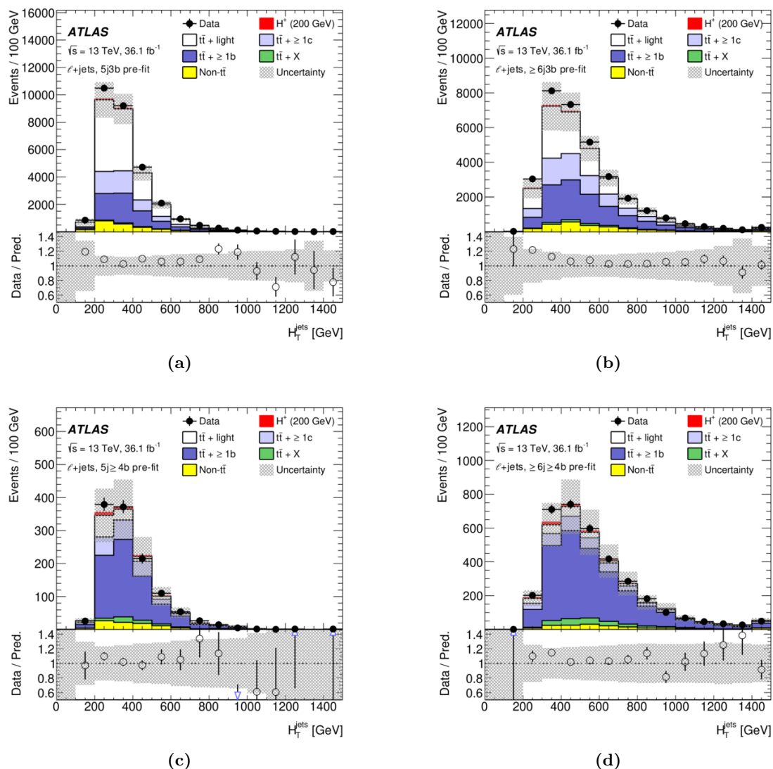
Figure 3. Distributions of the H_T^{\text{jets}} variable before the fit to the data in the four SRs of the \ell +jets channel: (a) 5j3b, (b) \geq 6j3b , (c) 5j \geq 4b , (d) \geq 6j \geq 4b . Each background process is normalised according to its cross-section and the normalisation of the t\bar{t} + \geq 1b and t\bar{t} + \geq 1c backgrounds corresponds to the prediction from POWHEG+PYTHIA8 for the fraction of each of these components relative to the total t\bar{t} prediction. The t\bar{t} + X includes contributions from t\bar{t}W , t\bar{t}Z and t\bar{t}H . In addition, the expectation for a 200 GeV signal is shown for a cross-section times branching ratio of 1 pb. The lower panels display the ratio of the data to the total prediction. The hatched bands show the pre-fit uncertainties. The level of agreement is improved post-fit due to the adjustment of the normalisation of the t\bar{t} + \geq 1b and t\bar{t} + \geq 1c backgrounds and the other nuisance parameters by the fit.
