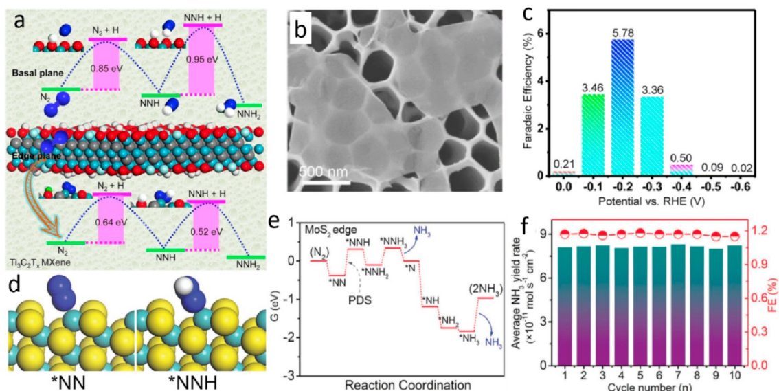
Figure 9. (a) Schematic structures and energies of the intermediates and transition states for NRR on the basal and edge planes. (b) SEM of ultrathin Ti_3C_2T_x NSs. (c) FEs obtained at various potentials. Reproduced with permission from ref 138. Copyright 2018 Elsevier. (d) The structures of *NN and *NNH on Mo-edge. (e) Free-energy profile for NRR at MoS_2 edge site. (f) Stability evaluation with 10 successive tests. Reproduced with permission from ref 139. Copyright 2018 Wiley-VCH Verlag GmbH & Co. KGaA, Weinheim.
