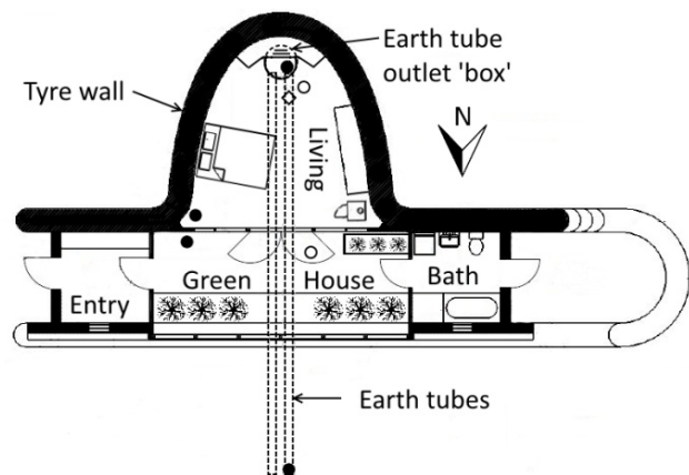
Figure 3: Floor plan of the Earthship building
