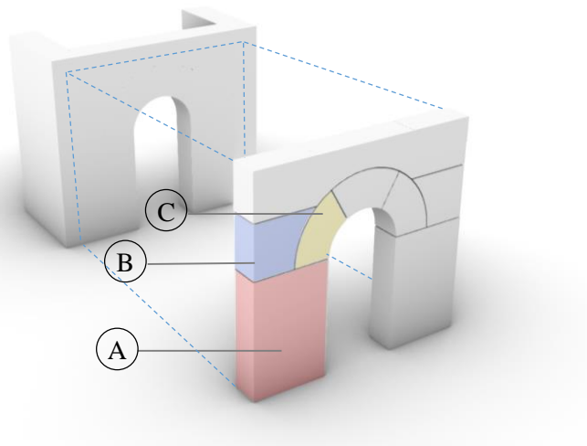
633 Figure 22. Geometry challenges in a regular cob wall with an opening. 1) Lift height- 3 axis 3D 634 printing; 2) Inclined 3-axis printing (corbelling); 3) Inclined 6-axis 3D printing.
