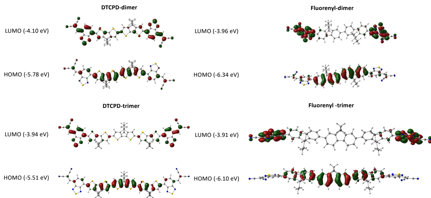
Figure 3. Molecular orbitals of the DTCPD- and fluorenyl-based dimers and trimers showing the HOMO and LUMO distributions. Calculations were done using the Amsterdam Density Functional package (ADF 2019.301).
