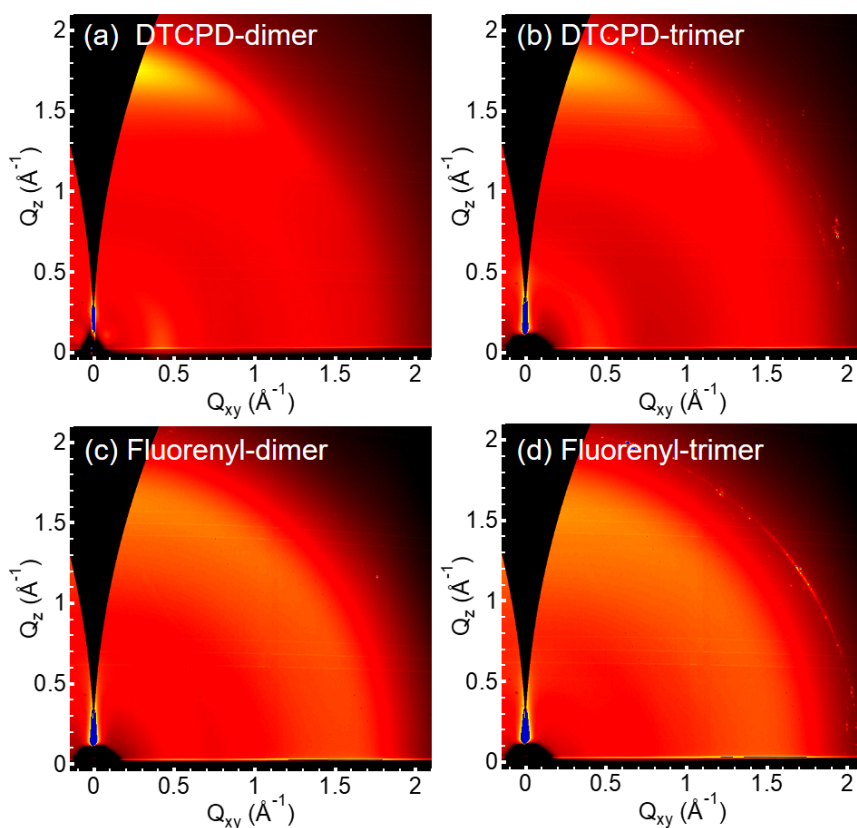
Figure 2. 2D GIWAXS patterns of neat films of DTCPD-dimer (a) and -trimer (b) and Fluorenyl-dimer (c) and -trimer (d) cast from chloroform solutions onto silicon substrates.
