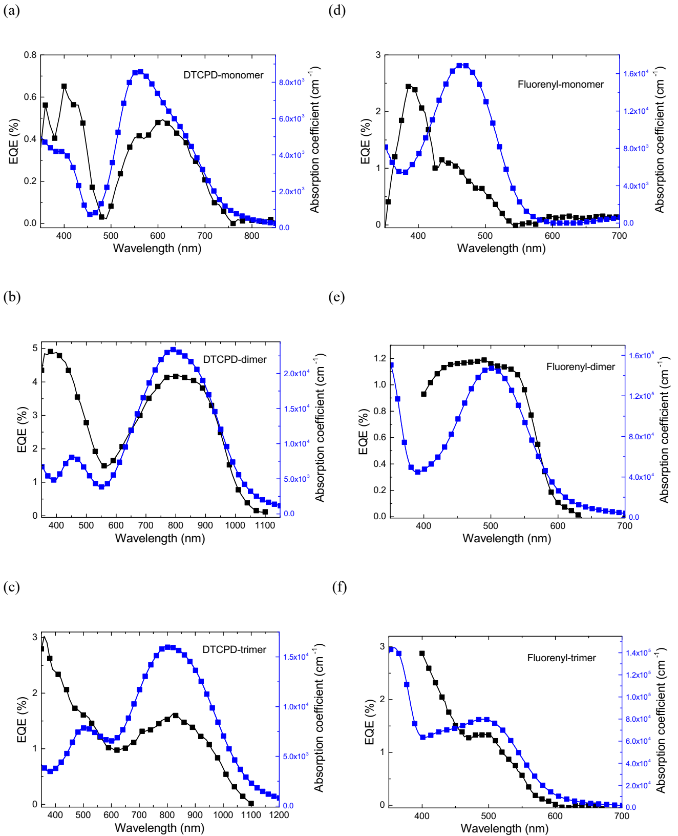
Figure 5. Film absorption spectra and external quantum efficiency (EQE) of homojunction devices with a structure of ITO/PEDOT:PSS/homojunction/Ca/Al composed of DTCPD-monomer (a), -dimer (b) and -trimer (c), and Fluorenyl-monomer (d), -dimer (e) or -trimer (f).
