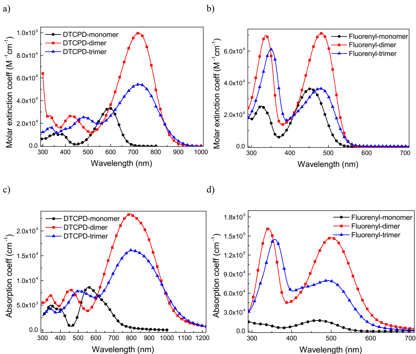
Figure 4. Molar extinction coefficient as a function of wavelength for solutions of the DTCPD (a) and fluorenyl (b) series, and absorption coefficient as a function of wavelength for films of the DTCPD (c) and fluorenyl (d) series.
