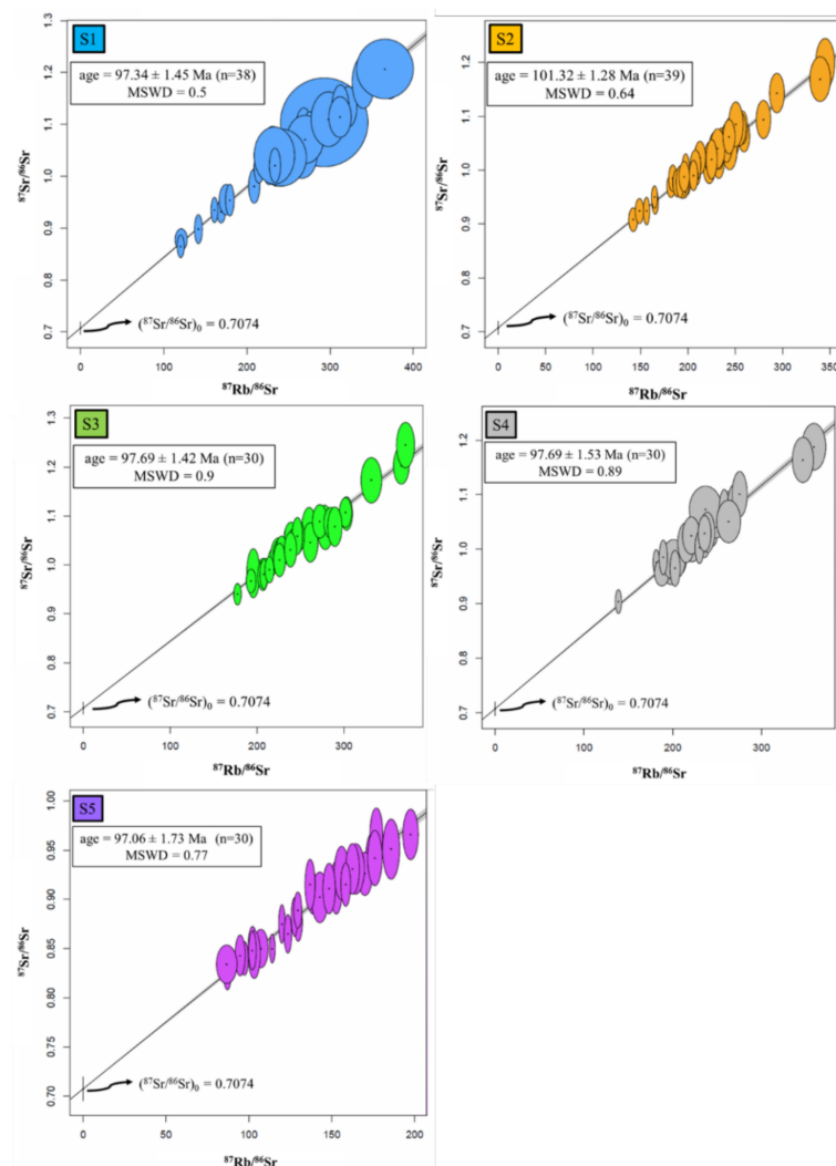
Figure 5. Isochron plots displaying glauconite bulk ages and related uncertainties ( 1\sigma is shown as ellipses and 2\sigma is indicated in the annotated boxes) as well as MSWD that is consistently < 1 for the glauconite separates of samples S1–S5 ( n = 167 ). Note that an initial seawater ^{87}\text{Sr}/^{86}\text{Sr} value of 0.7074 for the Cretaceous was used [48].
