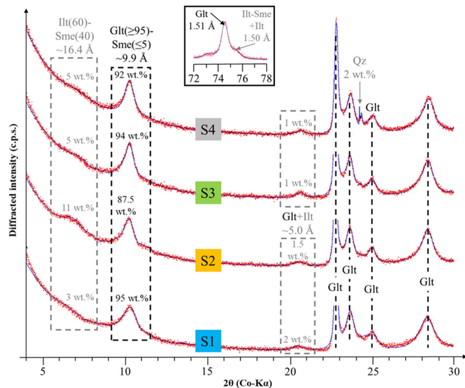
Figure 4. XRD patterns of separated glauconite powders (S1–S4) upon ethylene glycol solvation displaying characteristic peaks for glauconite (Glt-Sme), quartz (Qz), illite-smectite (Illt-Sme), and illite/muscovite (Illt), respectively. Red data points refer to measured diffracted intensities and blue curves mark Rietveld-based best-fitting lines.
