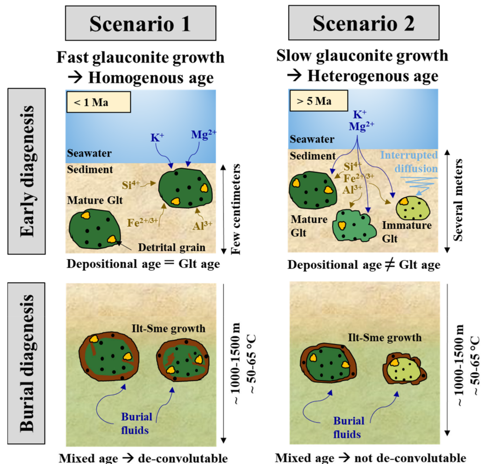
Figure 1. Schematic illustration of rapidly vs. slowly progressing glauconite (Glt) formation in shallow-marine sediments with corresponding effects on glauconite formation ages: Scenario 1 ( left panel ) assumes that the glauconite formation age is coeval or about equal to the sediment depositional age due to fast glauconitization at the sediment–seawater interface [13]. Scenario 2 ( right panel ) anticipates that the glauconite formation age is different compared to the sediment depositional age, reflecting the complexity of seawater/porewater evolution and local glauconite/sediment substrate interactions during slow glauconitization within the sedimentary column [22]. In both cases, the diagenetic intergrowth of illitic phases and the presence of inherited detrital grains can further affect the glauconite bulk ages.
