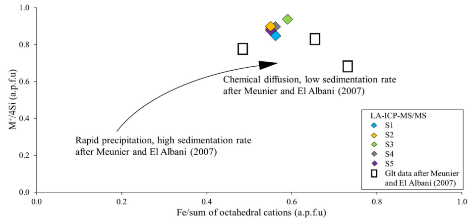
Figure 7. Plot of the average glauconite compositions obtained by LA-ICP-MS/MS analysis in the M^+/4Si vs. Fe/\text{sum of octahedral cations} diagram [22]. Slowly progressing glauconite formation is indicated, which is inconsistent with our glauconite ages measured by in situ Rb-Sr dating of glauconite grain separates.
