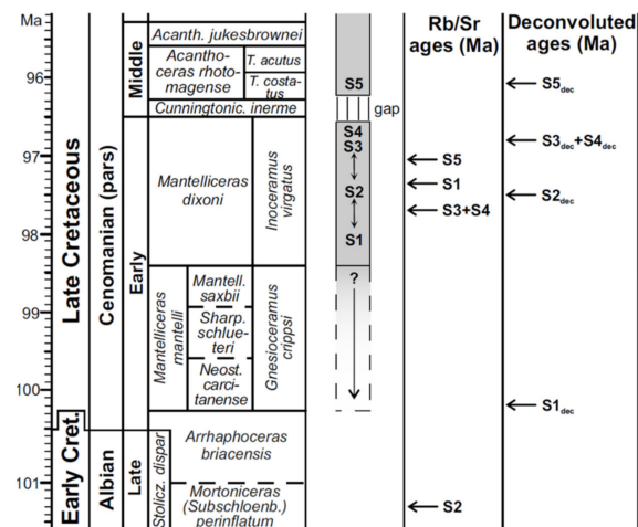
Figure 6. Bio-stratigraphic and geochronologic framework of the Langenstein section and absolute ages of samples S1–S5. The bio-stratigraphic position of the Langenstein section is based on Horna [16] and Wilmsen [29], starting in the late Early Cenomanian M. dixonii Zone (grey bar), with approximate positions of samples used in this study (note the stratigraphic gap in the Early–Middle Cenomanian boundary interval). The light-grey range bar with broken line indicates a potential downward extension of the section into the earliest Cenomanian, corroborated by the corrected age of sample S1. The measured Rb–Sr ages of samples S1–S5 generally overlap with the expected bio-stratigraphic age within analytical uncertainty (except for sample S2) but show no consistent stratigraphic age progression. The deconvoluted ages of samples S1–S5 are in stratigraphic order and fall within the expected M. dixonii and A. rhotomagense zones (note the outlier of sample S1 that suggests the presence of the lower M. mantelli Zone in the lowermost part of the Langenstein section, potentially reflecting an earlier Cenomanian transgression event). Absolute ages are after GTS 2020 [73] and cyclostratigraphic considerations; ammonite biostratigraphy is after Wright and Kennedy [28]).
