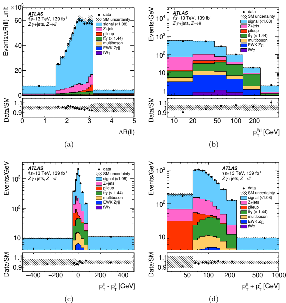
Figure 3. The measured (a) \Delta R(\ell, \ell) , (b) p_T^{\ell\ell\gamma j} , (c) p_T^{\ell\ell} - p_T^{\gamma} , and (d) p_T^{\ell\ell} + p_T^{\gamma} distribution (dots) in the signal region. The error bars represent the data statistical uncertainty; for most of the points, the error bars are smaller than the marker size and, thus, not visible. The MC simulation of the signal from SHERPA 2.2.11 (blue histograms) and various backgrounds are also included. The signal and background distributions are stacked to produce the figures. The variable bin width is taken into account in the vertical scale. The lower part of each figure shows the ratio of the data to the expected total SM distribution. The hatched band represents the statistical and systematic uncertainties of the SM background yields added in quadrature, excluding theory uncertainties of the signal.
