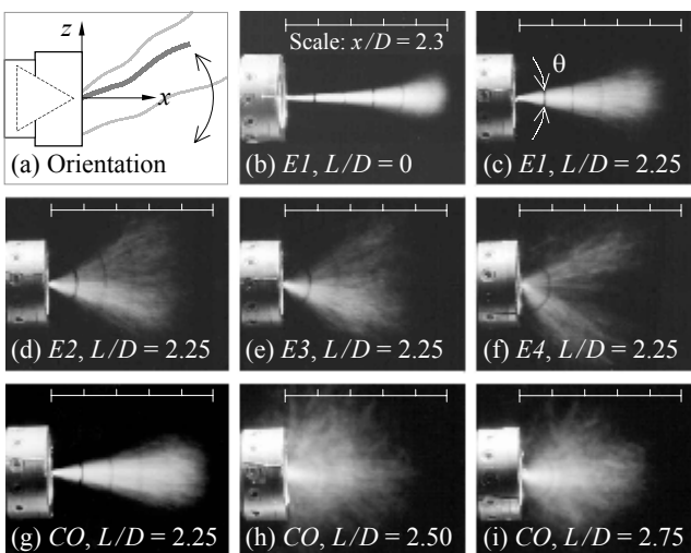
Figure 2. Flow visualisation of oscillating-jets: (a) nozzle orientation; (b)-(f), triangular orifice; (g)-(i), circular orifice. Each image is time average over 5 seconds. Re_1 = 50,000 .
