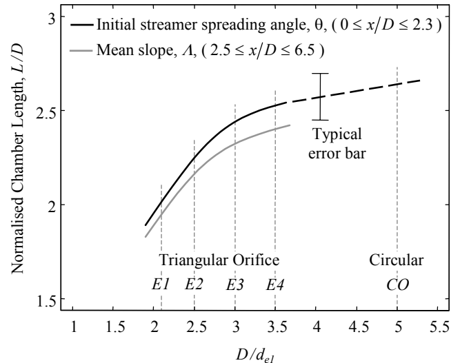
Figure 7. Domain of maximum streamer spreading angle, \theta , and mean slope, A , for Re_1 = 50,000 .
