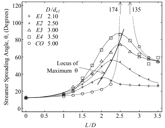
Figure 3. Initial streamer spreading angle, \theta , measured from the side-view photographs. +, \times , \Delta , \square , triangular orifice; \circ , circular orifice. Re_1 = 50,000 .
