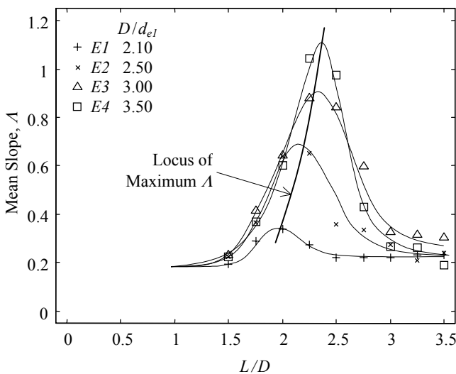
Figure 6. Mean slope, A , determined from the linear region of U_{\max-cl}/U_{cl} versus x/d_{el} data. +, x, Δ, □, triangular orifice. Re_1 = 50,000 .
