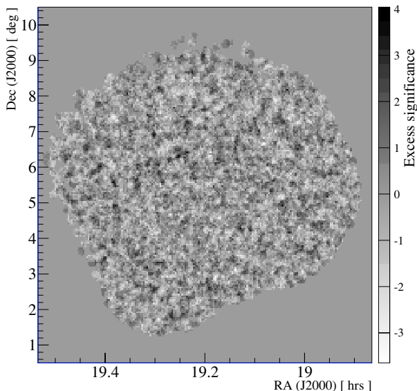
Fig. 6. Skymap of exp-test significance from Prah (1999) over the FoV (range and binning are the same as in Fig. 4 using the entire dataset). The 1D distribution of significances is well fitted by a Gaussian of mean \mu = 0.024 \pm 0.0007 and std. dev. \sigma = 0.965 \pm 0.005 .
