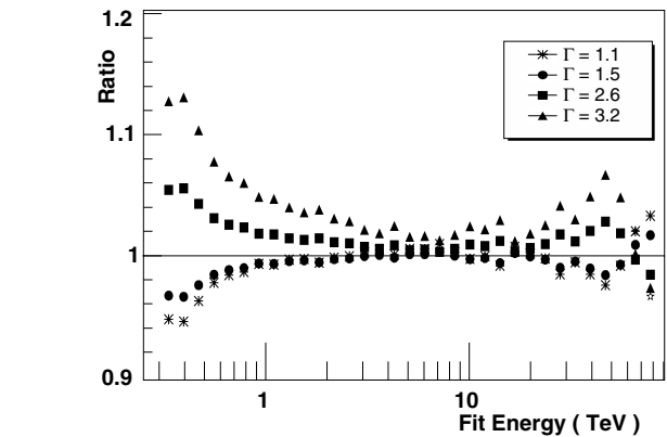
Fig. 17. The ratio of the reconstructed effective area (estimated assuming an photon index of 2.0) to the true effective area per energy bin, for true photon indices from 1.1 to 3.2, based on Monte Carlo simulations at 45^\circ zenith angle.
