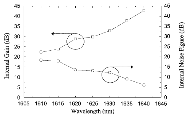
Fig. 4. Internal Raman gain and noise figure for various probe signal wavelengths (signal power, -10 dBm; pump peak power, 6.7 W).
