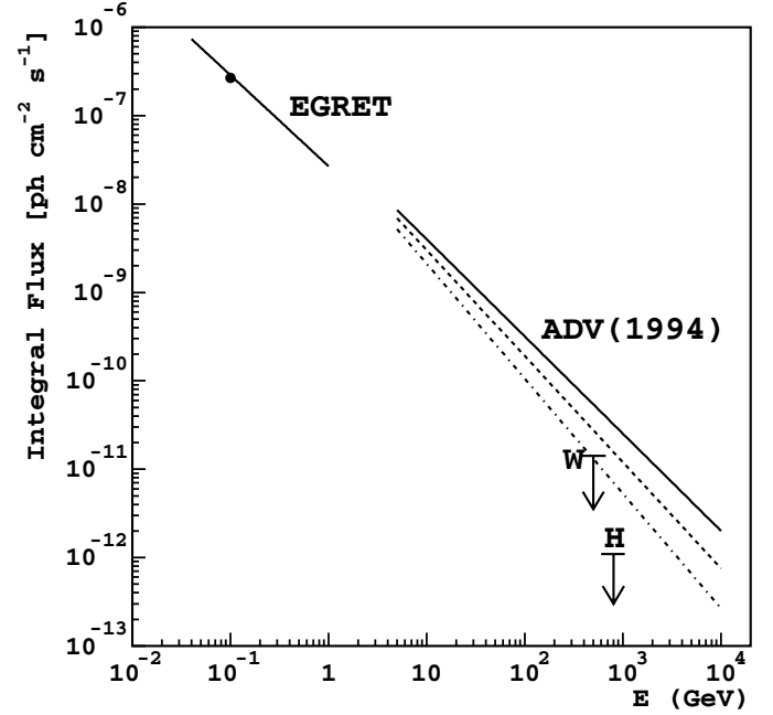
Fig. 5. Upper limits for 3EG J0634+521 (Monoceros Loop/Rosette Nebula interaction region) from the present work (H) and a previous measurement by the Whipple telescope (W) (see text for reference). We also show the measured EGRET integral flux and the expected integral \gamma -ray fluxes from \pi^\pm -decay based on the predictions of the ADV model and considering a mean matter density of the target (Rosette Nebula) of n \approx 40 cm ^{-3} . The solid, dashed and dash-dotted lines represent the predictions for three different assumptions on the spectral index of the differential energy spectrum of a population of shock-wave-accelerated protons ( dN/dE \propto E^{-\alpha+1} ); \alpha = 2.1, 2.2 and 2.3 , respectively.
