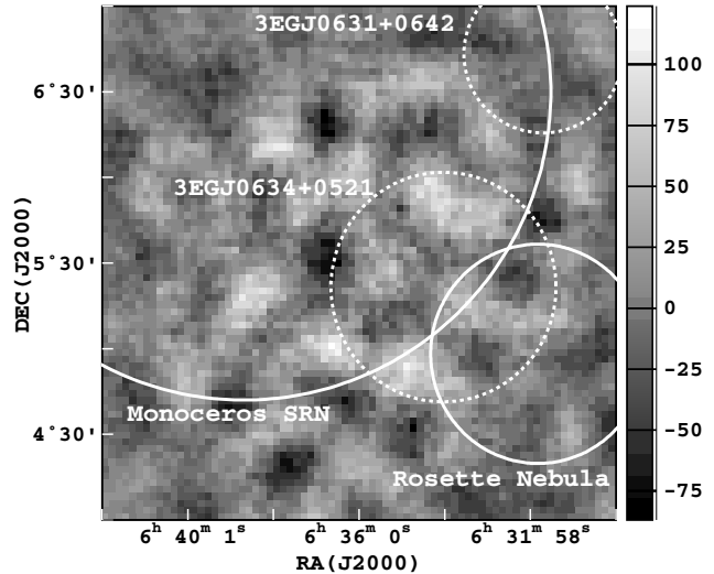
Fig. 4. 3^\circ \times 3^\circ smoothed sky map of the TeV excess events coming from the direction of the Monoceros Loop SNR (bin size: 0.04^\circ \times 0.04^\circ ). At each bin the excess is estimated using the ring background model described in the text with a point-like source search window of \theta = 0.13^\circ . Superimposed are the approximate extents of the Monoceros Loop and Rosette Nebula and the 95% error circles of the EGRET sources 3EG J0634+0521 and 3EG J0631+0642.
