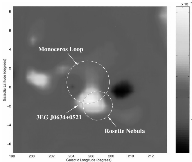
Fig. 2. EGRET detection plot from Jaffe et al. (1997). Shown are the approximate extension and position of the Monoceros Loop (big circle) and of the Rosette Nebula (small circle).
