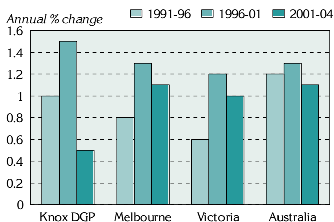
Figure 1: Annual population change, Knox DGP‡, Melbourne, Victoria and Australia, 1991 to 1996, 1996 to 2001 and 2001 to 2004
