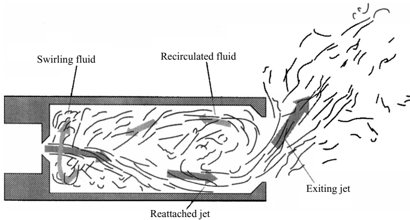
FIGURE 1. Conjectured flow structure of a simple FPJ nozzle comprising an orifice-type inlet and a chamber-lip configuration (Ch-L). Re_d = 15000 , D/d = 6.03 , d = 7.3 mm, D_1 = 44 mm, L = 114 mm, D_2 = 35 mm (Nathan et al. 1998). Reprinted with permission.
