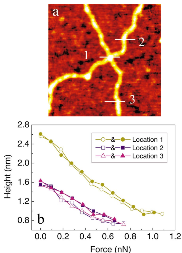
FIG. 4. (Color) (a) Topography of two crossed DNA molecules with A_{sp}=0.810 V. Image size: 200\text{ nm} \times 200\text{ nm} . (b) The height-force curves taken at three different locations as indicated in (a). The open and the corresponding solid square, triangle, and circle denote approaching and retracting processes, respectively.
