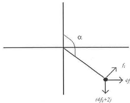
Figure 3.1: The Gribov pendulum
