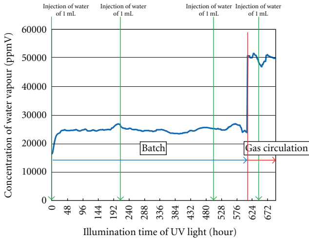
FIGURE 18: Concentration change in water vapour during the CO 2 reduction experiment by batch type and gas circulation type reactor with illumination time of UV light (injection of water of 1.00 mL many times).
