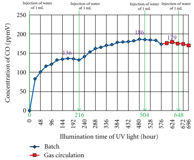
FIGURE 17: Concentration change in produced CO with illumination time of UV light (injection of water of 1.00 mL many times).
