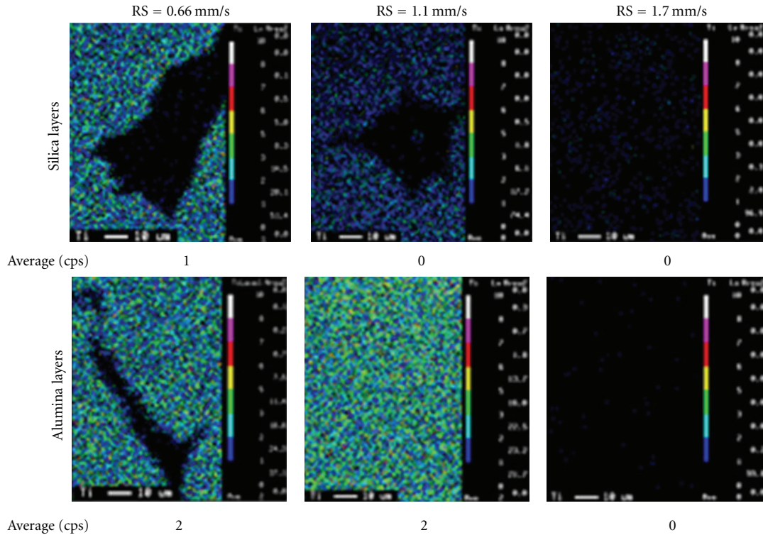
FIGURE 7: EPMA images of \text{TiO}_2 film prepared under various RS conditions.
