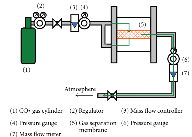
FIGURE 4: Arranged CO 2 reduction and permeation experimental system for CO 2 permeation experiment.
