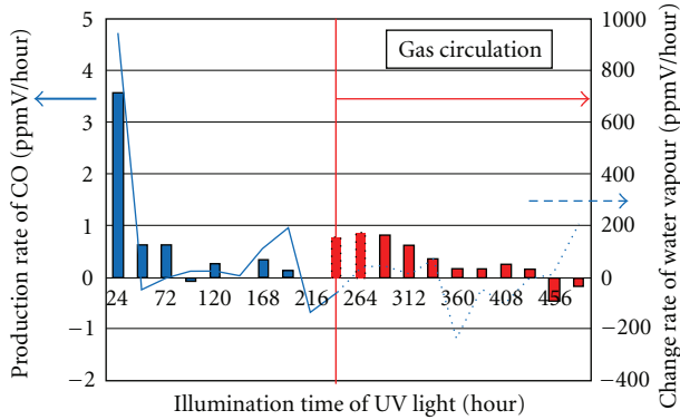
FIGURE 21: Change in production rate of CO and change rate of water vapour with illumination time of UV light for the amount of water injected of 1.00 mL.
