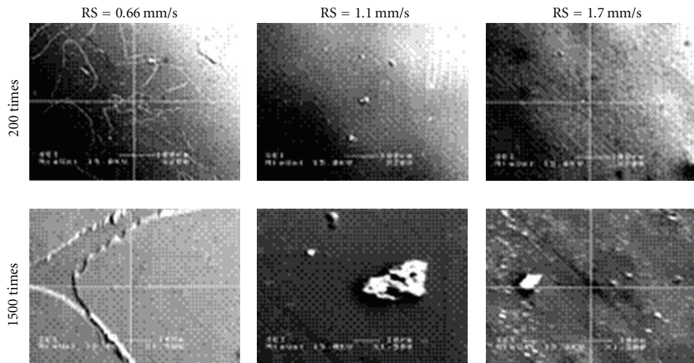
FIGURE 6: SEM images of TiO 2 film coated on alumina layer prepared under various RS conditions.
