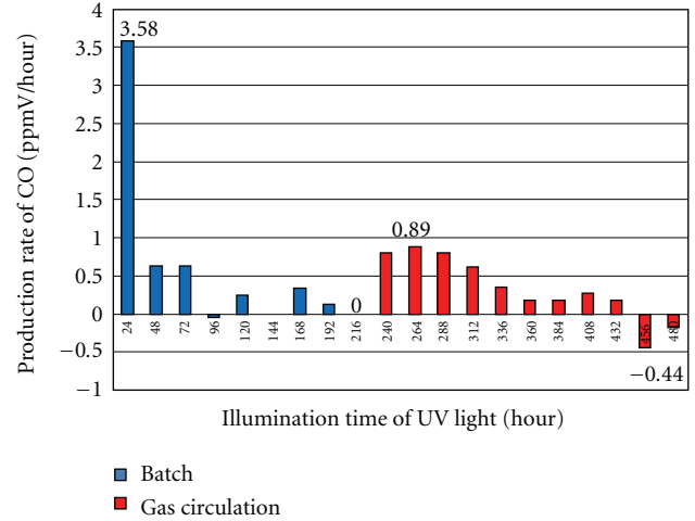
FIGURE 15: Change in production rate of CO with illumination time of UV light (injection of water of 1.00 mL at the start of CO 2 reduction experiment).
