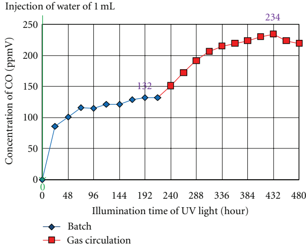
FIGURE 14: Concentration change in produced CO with illumination time of UV light (injection of water of 1.00 mL at the start of CO 2 reduction experiment).
