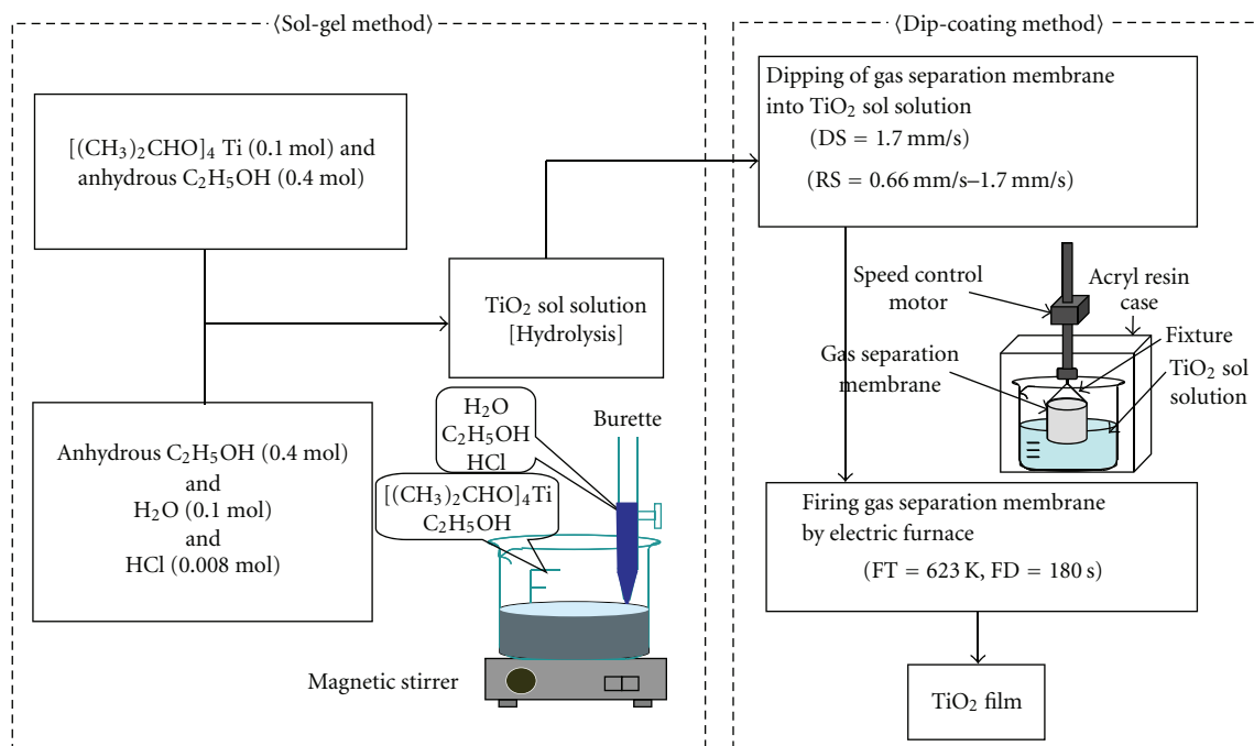
FIGURE 1: Sol-gel and dip-coating method to prepare \text{TiO}_2 film in this study.
