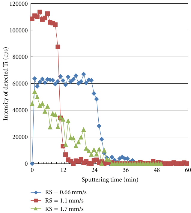
FIGURE 8: Intensity distributions of detected Ti in silica layer.
