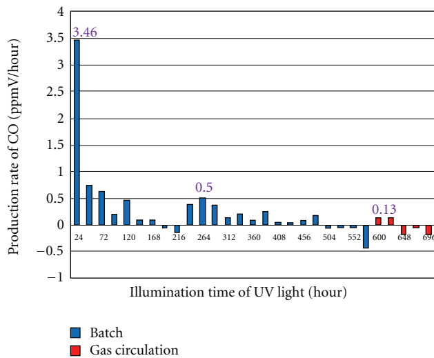
FIGURE 19: Change in production rate of CO with illumination time of UV light (injection of water of 1.00 mL many times).
