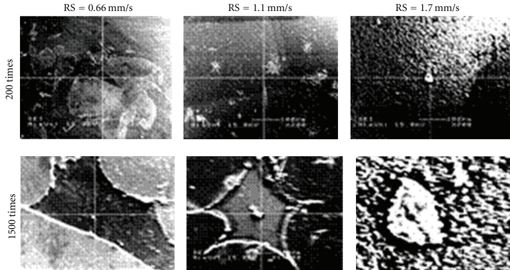
FIGURE 5: SEM images of TiO 2 film coated on silica layer prepared under various RS conditions.
