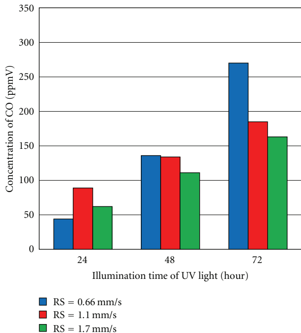
FIGURE 10: Concentration change in produced CO with illumination time of UV light for several TiO 2 film prepared under conditions of different RS.
