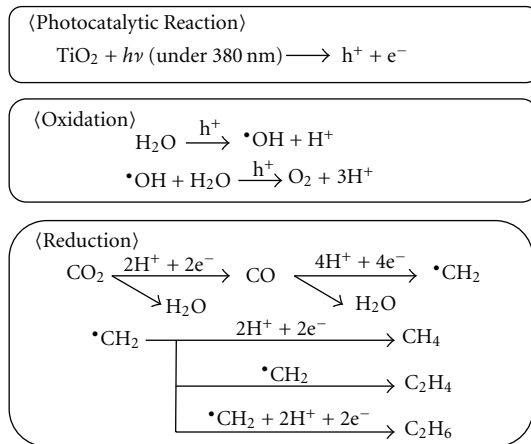
FIGURE 11: Reaction scheme of CO 2 reduction into fuel by TiO 2 photocatalyst.
