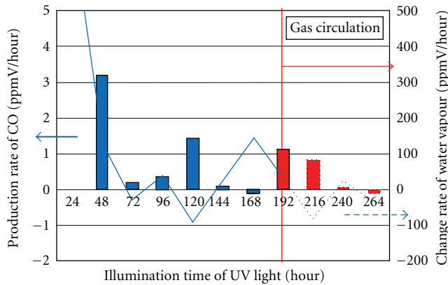
FIGURE 22: Change in production rate of CO and change rate of water vapour with illumination time of UV light for the amount of water injected of 3.00 mL.
