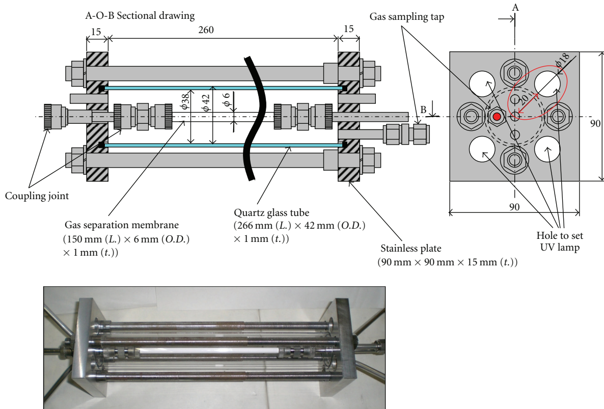
FIGURE 2: CO 2 reduction reactor composed of TiO 2 film coated on gas separation membrane (UV lamp is removed from this figure for understanding the inside of CO 2 reduction reactor).
