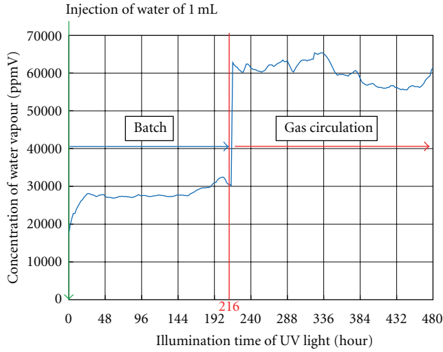
FIGURE 16: Concentration change in water vapour during the CO 2 reduction experiment by batch type and gas circulation type reactor with illumination time of UV light (injection of water of 1.00 mL at the start of CO 2 reduction experiment).
