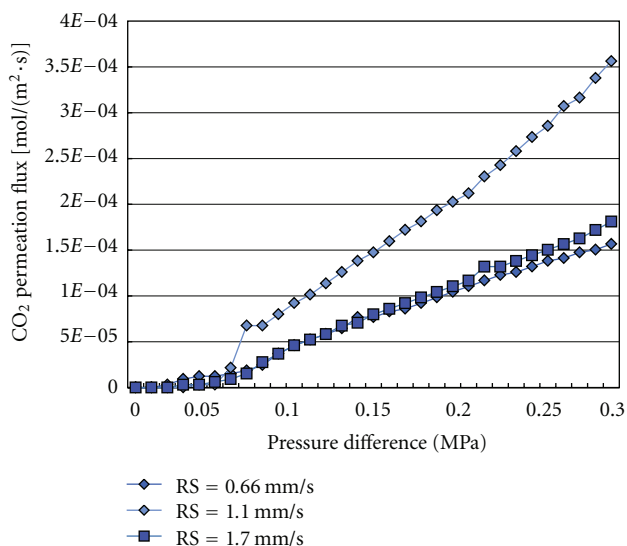
FIGURE 12: Relationship between CO 2 permeation flux and pressure difference for several TiO 2 film prepared under various RS conditions.
