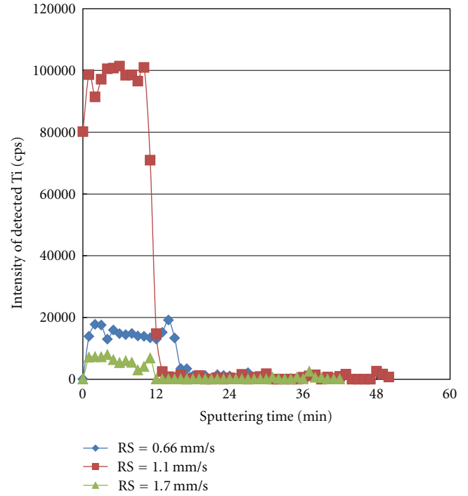
FIGURE 9: Intensity distributions of detected Ti in alumina layer.
