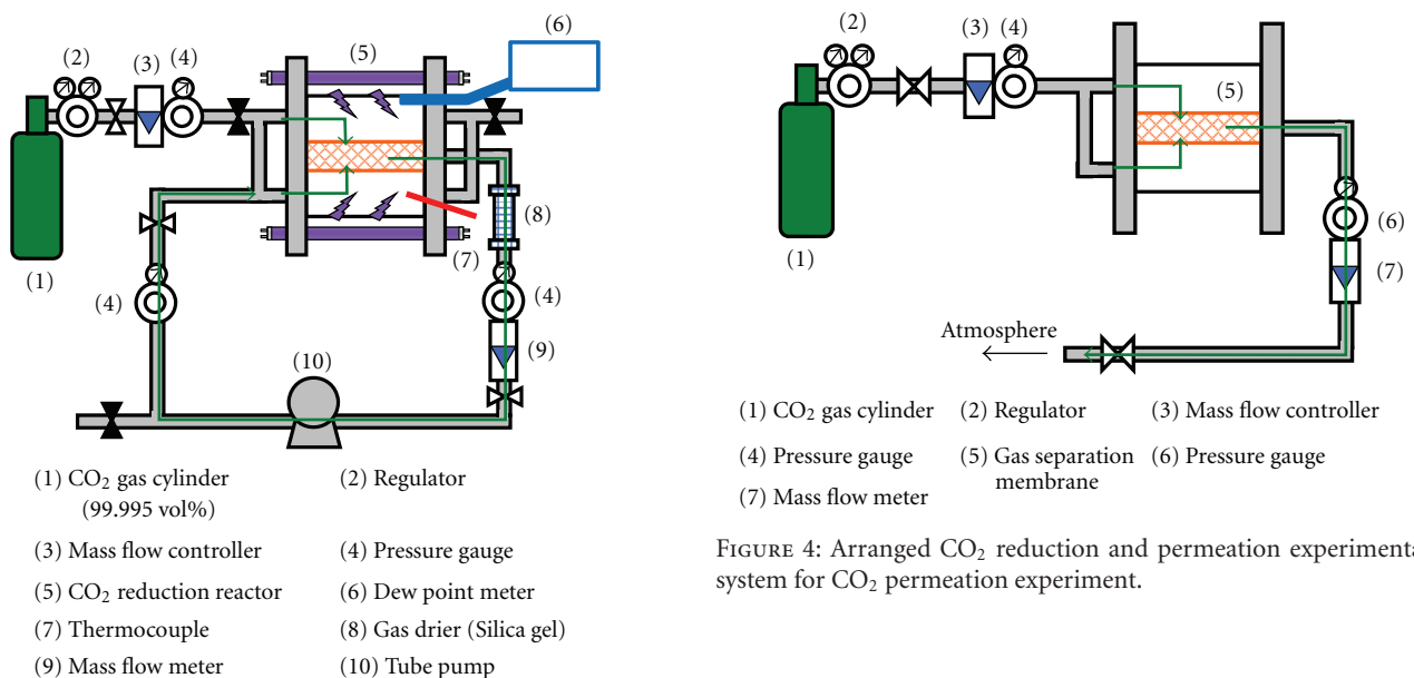
FIGURE 3: CO 2 reduction and permeation experiment system.
