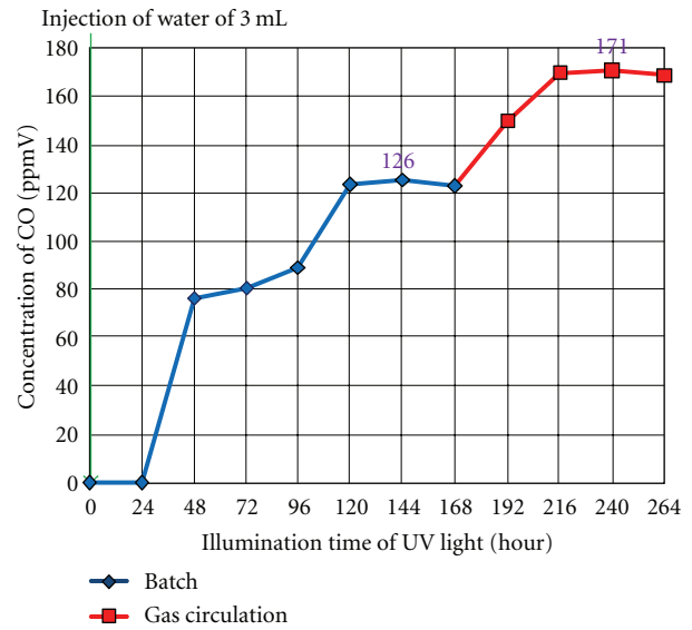
FIGURE 20: Concentration change in produced CO with illumination time of UV light (injection of water of 3.00 mL at the start of CO 2 reduction experiment).
