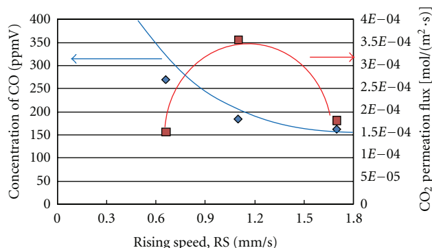
FIGURE 13: Comparison of the results between concentration of produced CO and CO 2 permeation flux for each condition.
