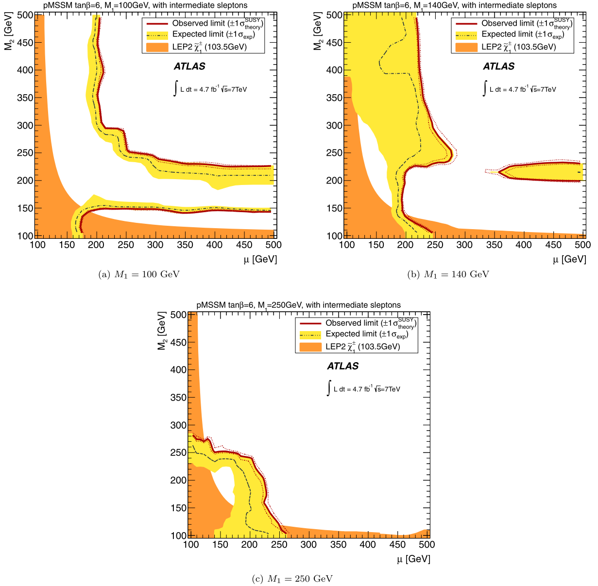
Fig. 3. 95% CL exclusion limits in the \mu – M_2 mass plane of the pMSSM for (a) M_1 = 100 GeV, (b) M_1 = 140 GeV and (c) M_1 = 250 GeV. The dashed and solid lines show the 95% CL s expected and observed limits, respectively, including all uncertainties except for the theoretical signal cross-section uncertainty (PDF and scale). The solid band around the expected limit shows the \pm 1\sigma result where all uncertainties, except those on the signal cross-sections, are considered. The \pm 1\sigma lines around the observed limit represent the results obtained when moving the nominal signal cross-section up or down by the \pm 1\sigma theoretical uncertainty.
