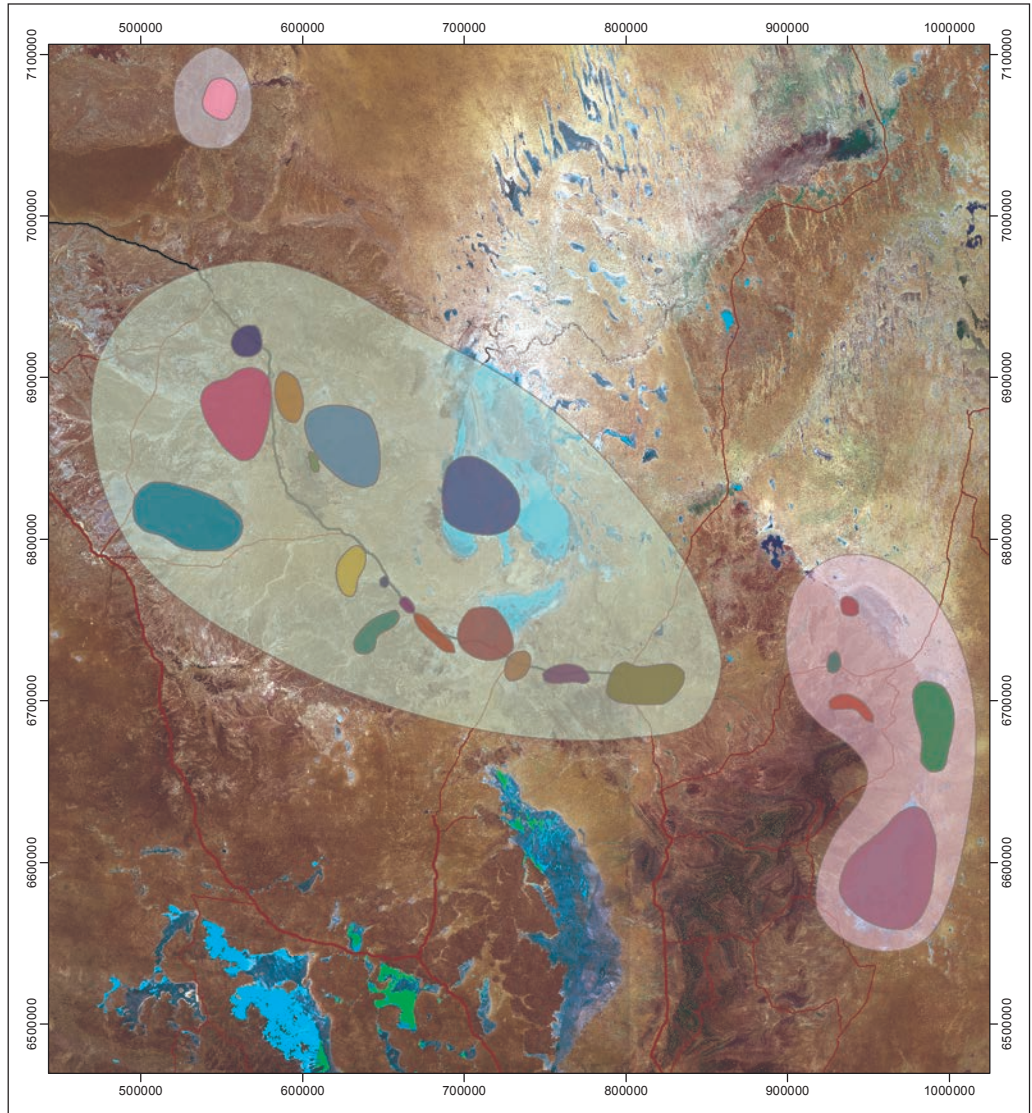
Figure 2.1: GAB spring supergroup and complex distribution in South Australia
