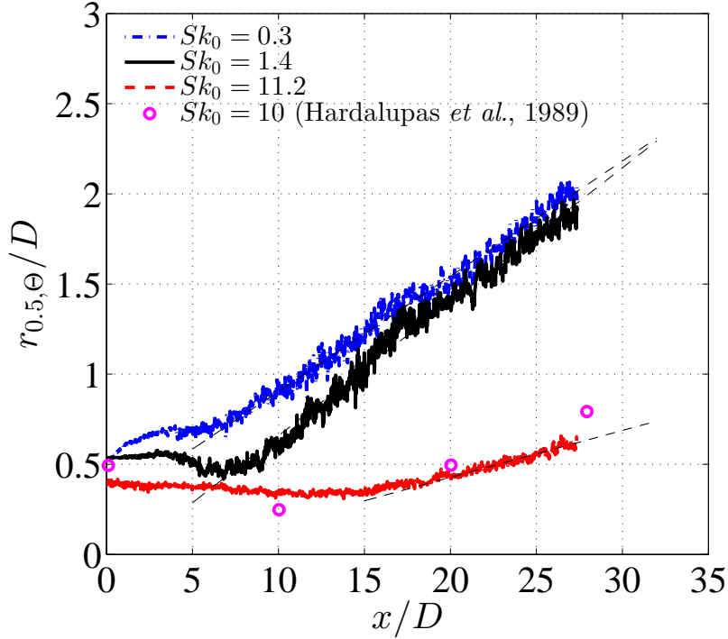
FIGURE 15. Axial evolution of the concentration half-width.
