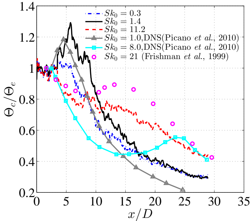
FIGURE 12. Axial evolution of the centreline concentration decay.
