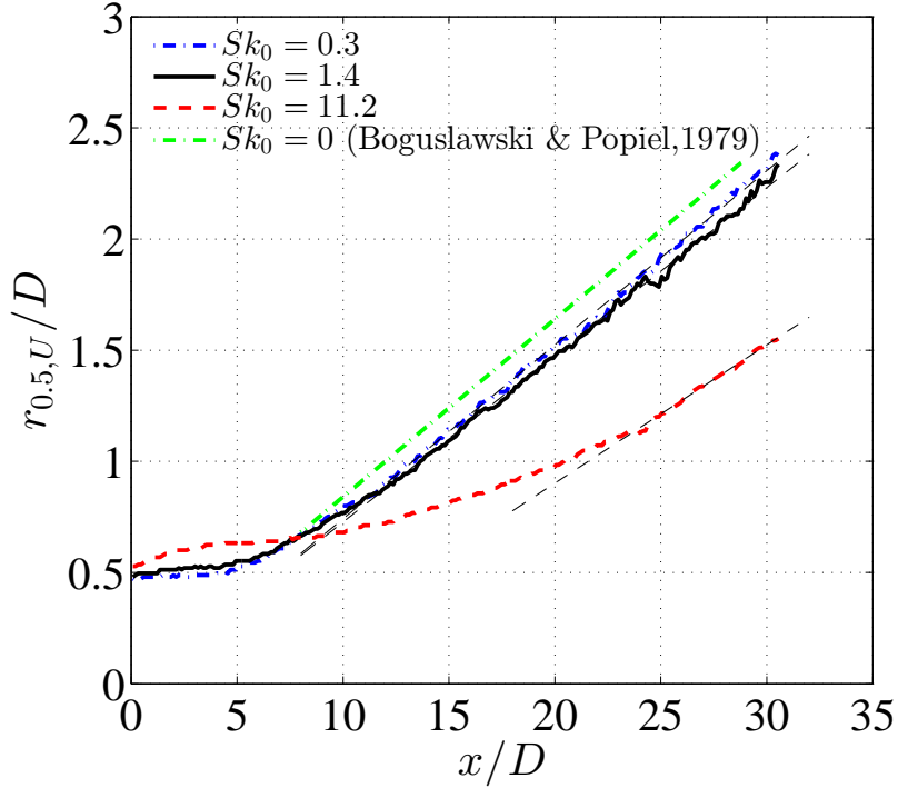
FIGURE 14. Axial evolution of the velocity half-width.
