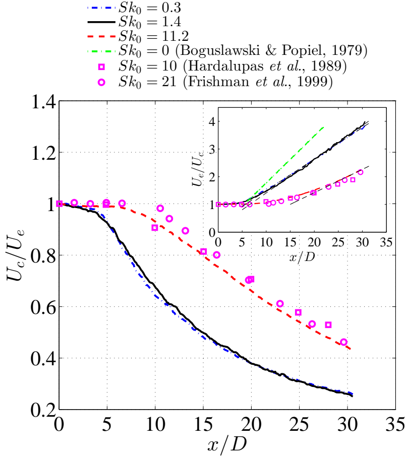
FIGURE 10. Axial evolution of the centreline velocity decay. The inset shows the axial evolution of the inverse centreline velocity.
