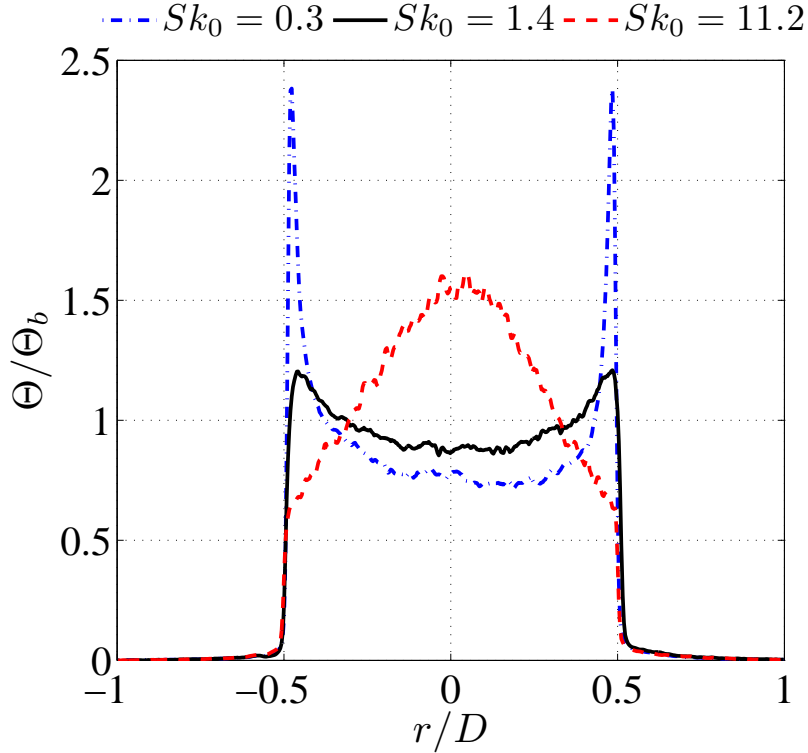
FIGURE 7. Radial concentration profile at the jet exit.
