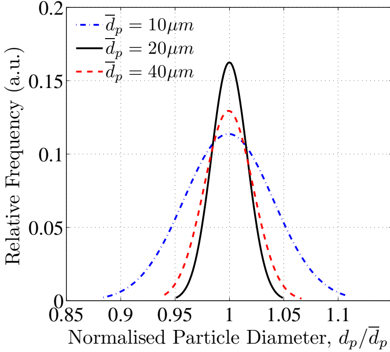
FIGURE 2. Particle size distribution.
