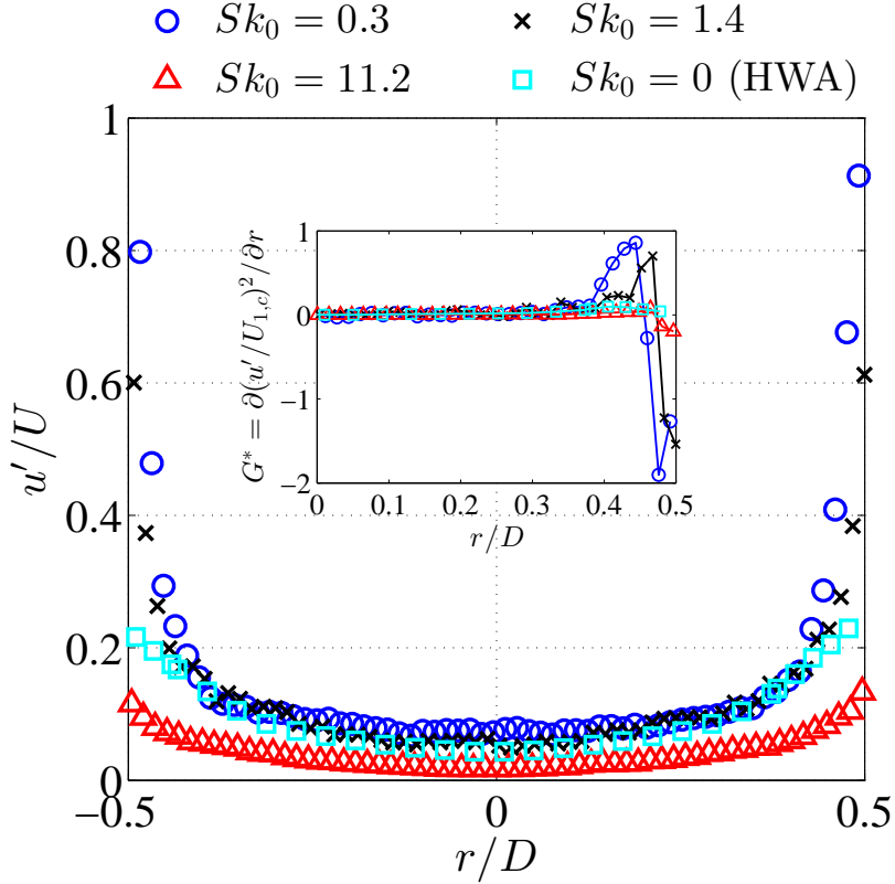
FIGURE 6. Radial profiles of the normalised r.m.s. of the axial velocity ( u'/U ) measured at the jet exit. The inset presents the radial gradient of the square of the normalised r.m.s. axial velocity, G^* , at the jet exit. The single-phase ( Sk_0 = 0 ) measurements were performed with hot-wire anemometry at Re_D = 10,000 . For flow conditions of the two-phase measurements, see table 3.
