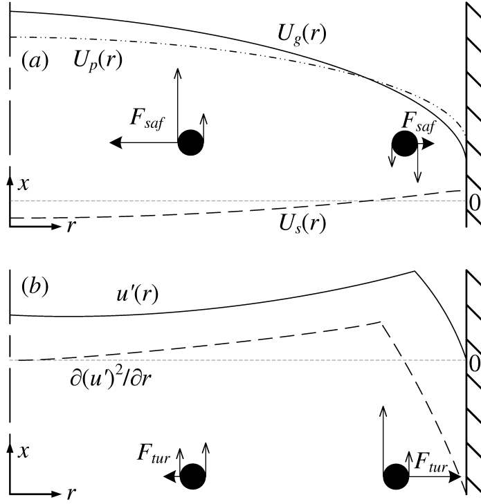
FIGURE 8. Schematic diagram of (a) Saffman-lift and (b) turbophoresis acting on particles in a fully-developed pipe flow. Here F_{saf} is the Saffman-lift force, F_{tur} is the turbophoretic force, and U_s = U_p - U_g is the particle slip velocity. Diagram is not to scale (proportions exaggerated for clarity).
