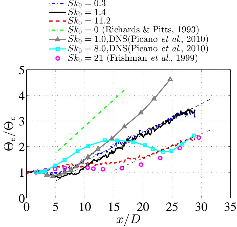
FIGURE 13. Axial evolution of the inverse centreline concentration.
