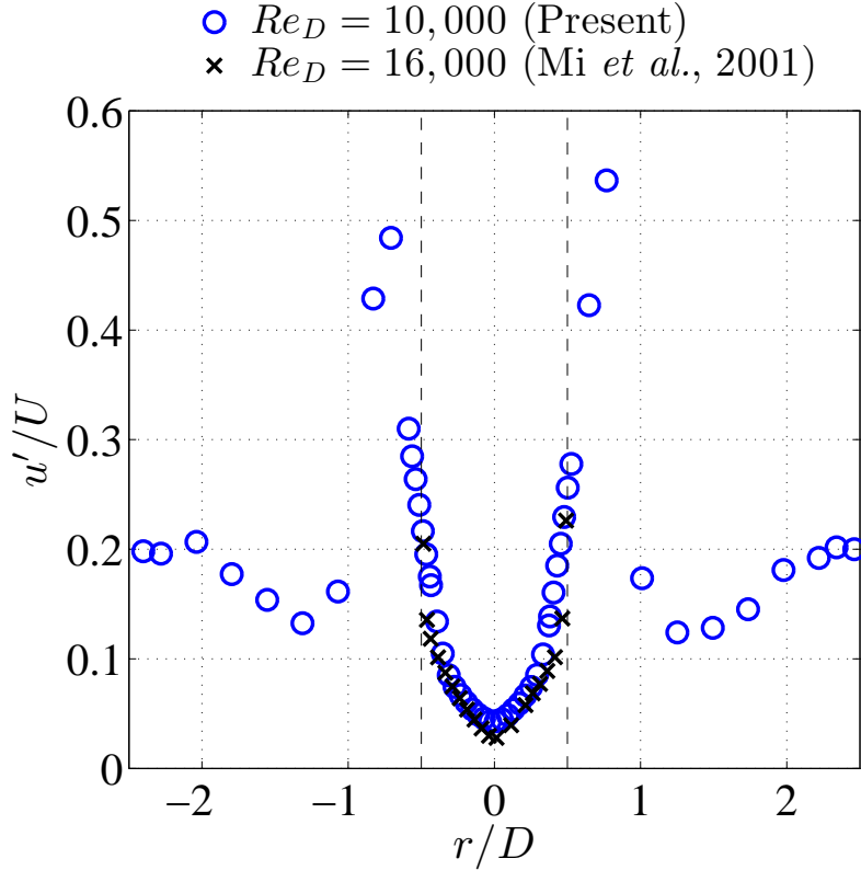
FIGURE 4. Single-phase r.m.s. axial velocity at the jet exit as recorded by hot-wire anemometry, both for the present jet with co-flow, and for a previous jet without co-flow.
