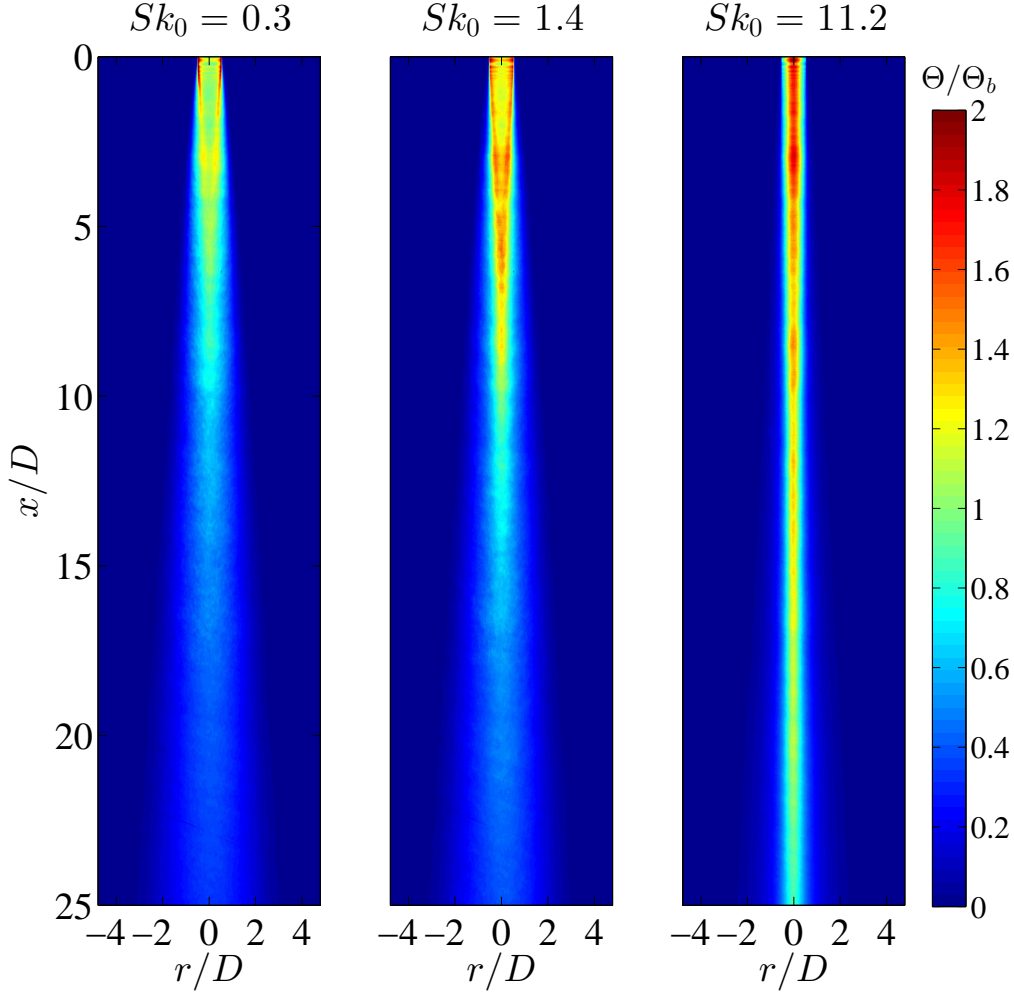
FIGURE 9. The mean distributions of particle concentration normalised by the bulk-mean exit values ( \Theta/\Theta_b ) for three values of Sk_0 .
