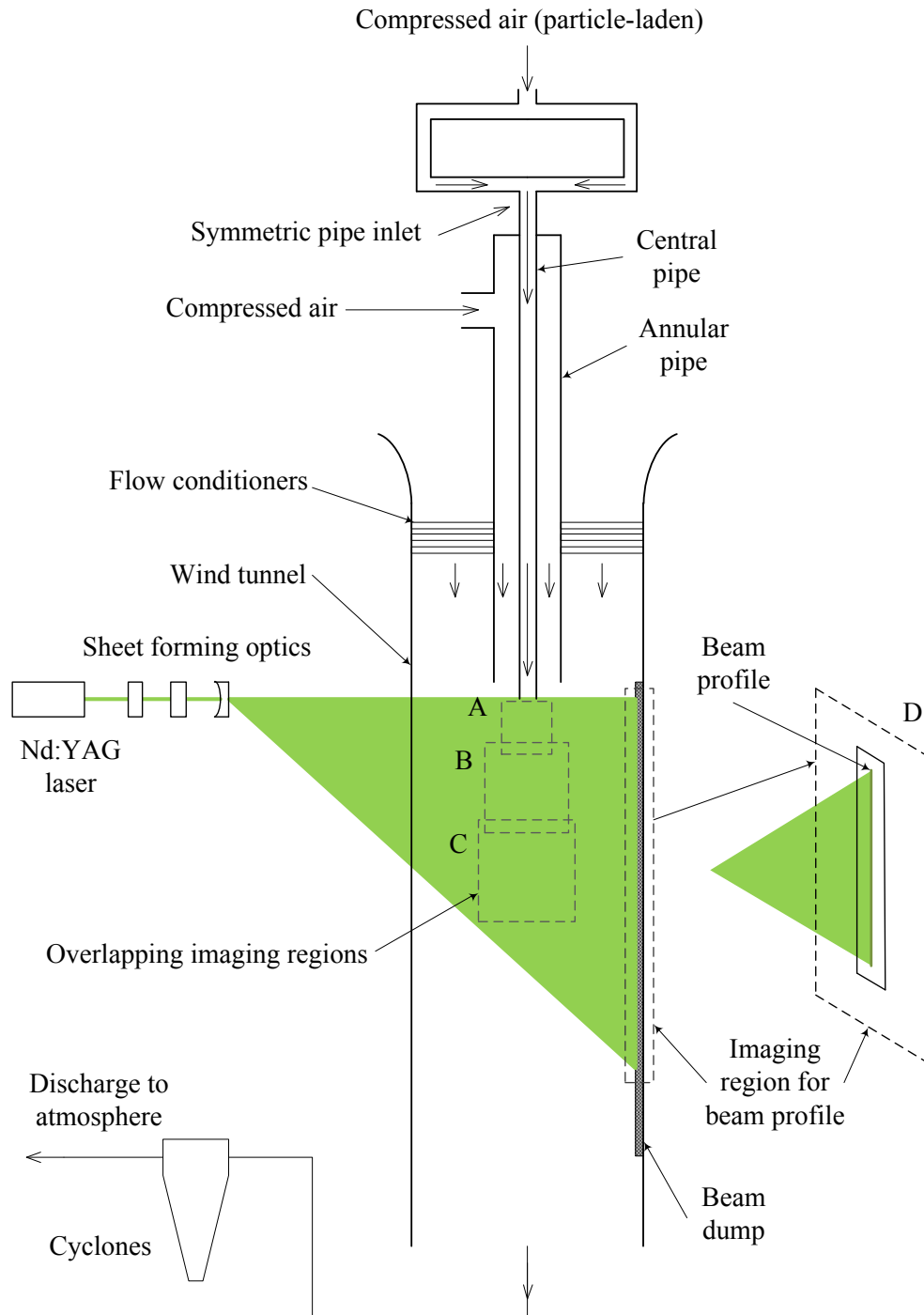
FIGURE 1. Experimental arrangement.
