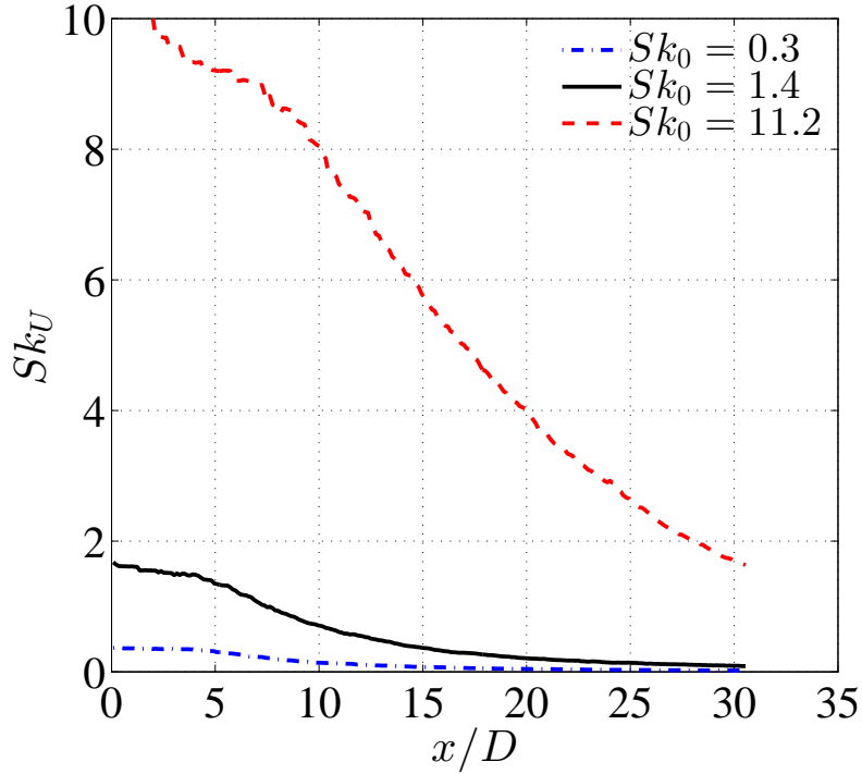
FIGURE 11. Variation of local Stokes number with streamwise distance from the jet exit.
