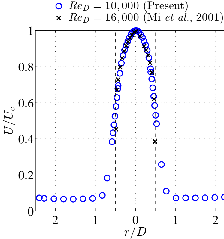
FIGURE 3. Single-phase mean axial velocity at the jet exit as recorded by hot-wire anemometry, both for the present jet with co-flow, and for a previous jet without co-flow.
