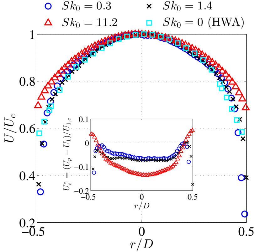
FIGURE 5. Radial profiles of mean axial velocity at the jet exit. The inset shows radial profiles of the quasi-slip velocity, U_s^* , which is the difference between the axial components of the single-phase gas velocity and the particle velocity. The single-phase ( Sk_0 = 0 ) measurements were performed with hot-wire anemometry at Re_D = 10,000 . For flow conditions of the two-phase measurements, see table 3.
