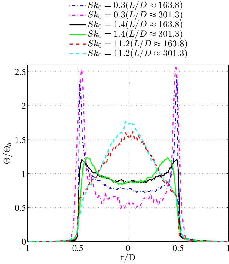
FIGURE 16. Comparison of exit concentration for two different pipe lengths at all investigated Stokes numbers.
