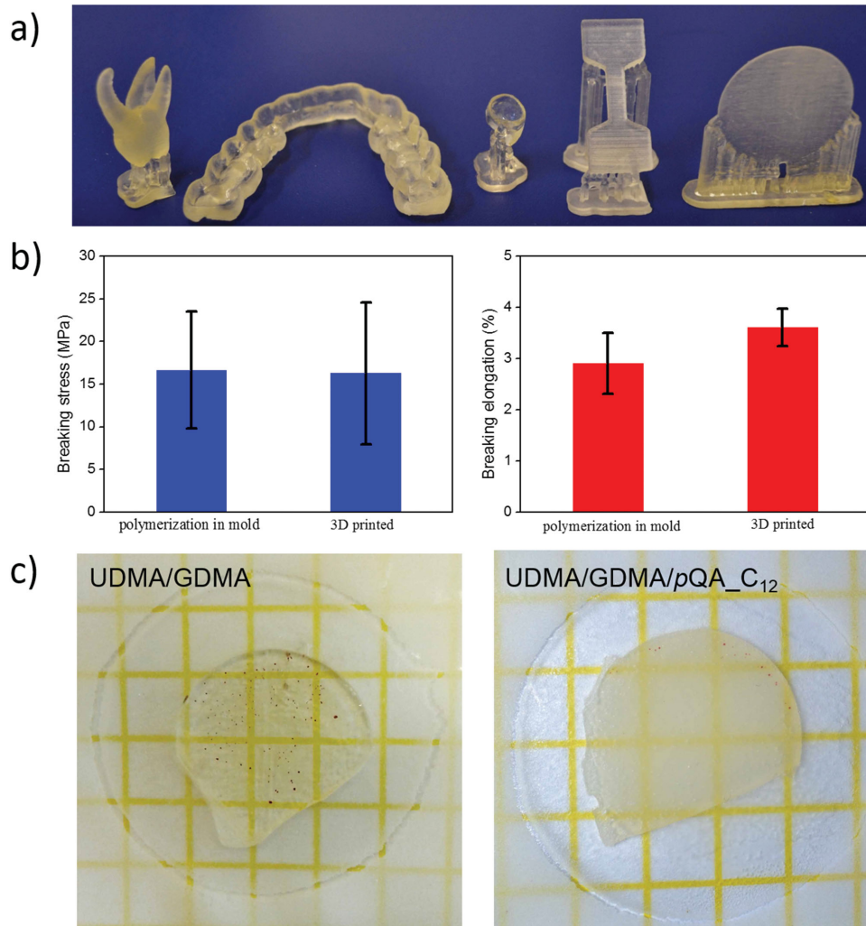
Figure 6. Object examples and properties of 3D printed, 25 wt% pQA C12 in a polymer-incorporated SIPN resin of UDMA/GDMA. a) 3D printed dental appliances or models (from left to right: molar tooth, clear splint, crown, tensile test bar, contact-killing test disc) based on polymerized positively charged compounds incorporated in an SIPN resin; b) tensile properties of 25 wt% pQA C12 in a polymer-incorporated SIPN system of UDMA/GDMA 3D printed tensile test bar and a test bar prepared in a polymerization mold by conventional photoillumination; and c) comparison of the contact-killing efficacy of a 3D printed 25 wt% pQA C12 in a polymer-incorporated SIPN system of UDMA/GDMA disc for S. mutans NS in the Petrifilm plate counting system with the one of a UDMA/GDMA disc (challenge number equals 30 CFUs cm -2 ). Presence of CFUs (red dots) on the UDMA/GDMA disc versus the absence of CFUs on the UDMA/GDMA/pQA C12 disc indicates that the bacterial contact-killing ability of the material is preserved upon 3D printing.
